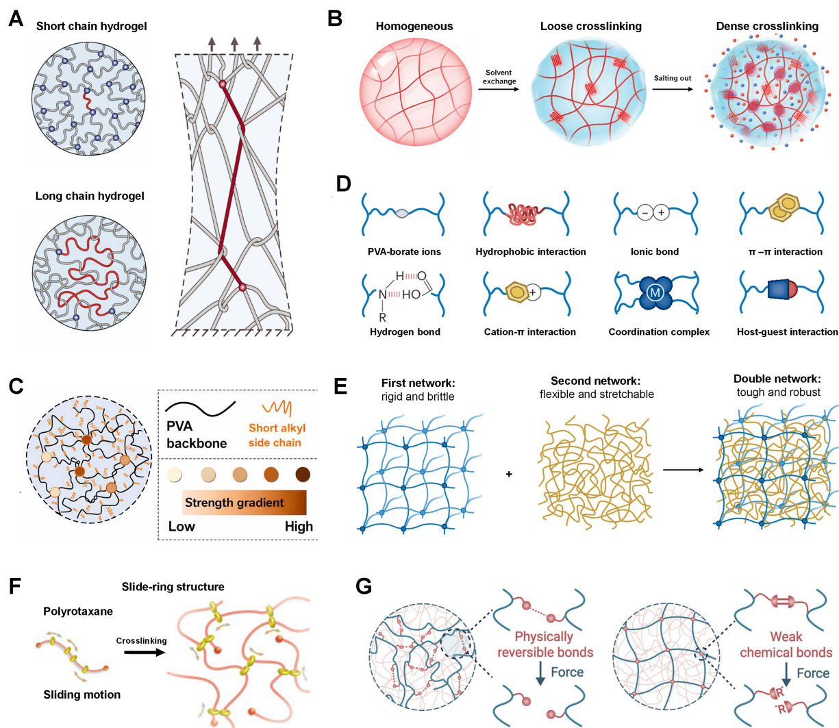
Figure 2. Molecular/chain-level structure strategy. (A) Chain flexibility tuned by molecular weight and degree of polymerization [40,52] . Copyright 2021, The American Association for the Advancement of Science; Copyright 2022, Wiley-VCH; (B) Crosslinking density [53] . Copyright 2023, Wiley-VCH; (C) Branching and side-chain structures [41] . Copyright 2021, American Chemical Society; (D) Self-assembly and noncovalent interactions; (E) Double/multiple network structures. (D and E) are reprinted with permission from Ref. [34] . Copyright 2024, Springer Nature; (F) Slide-ring and fully sliding structures [54] . Copyright 2010, Elsevier; (G) Sacrificial network design [55] . Copyright 2025, Innovation Press. PVA: Poly(vinyl alcohol).
