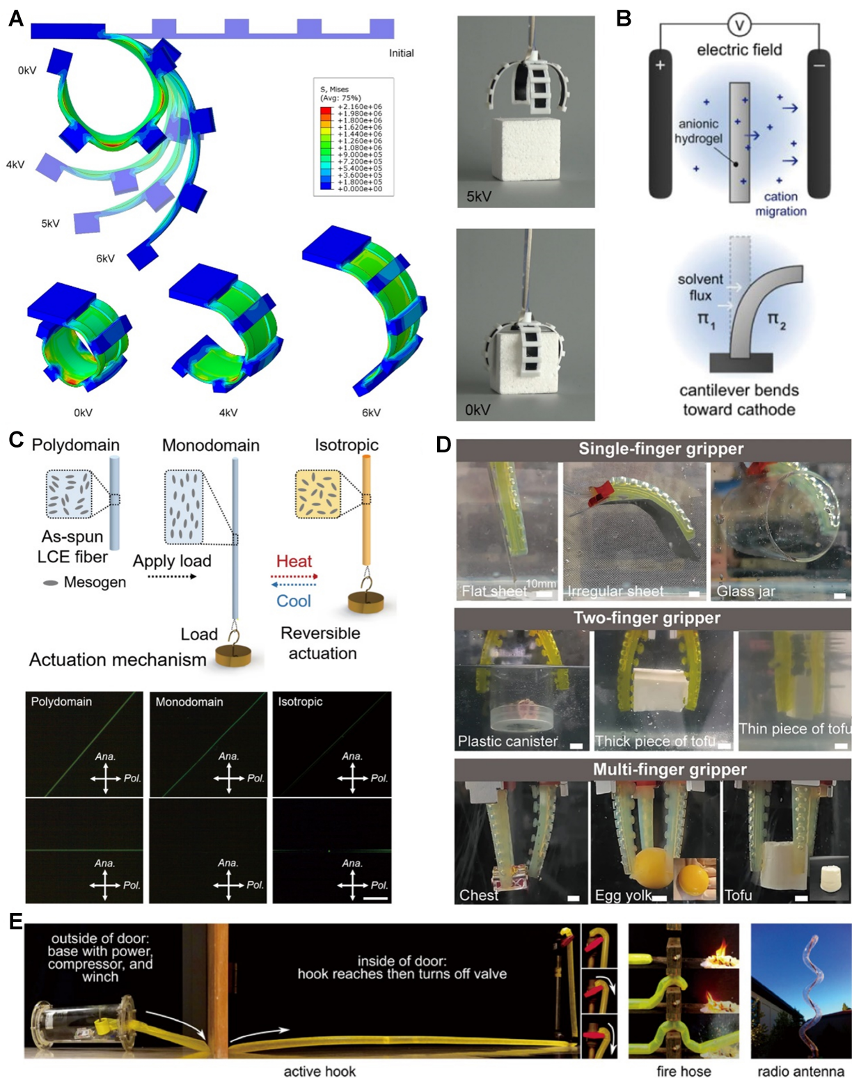
Figure 10. Actuation mechanism and motion complexity and structural design. (A) DEA soft gripper grips a cube [295] . Copyright 2019, Elsevier; (B) Illustration of electro-osmotic actuation mechanism [296] . Copyright 2022, American Chemical Society; (C) Top: Actuation mechanism of LCE fiber; bottom: POM images of polydomain, monodomain, and isotropic states of LCE microfibers observed at two different angles with respect to the analyzer [300] . Copyright 2021, The American Association for the Advancement of Science; (D) Designed and manufactured single-finger, two-finger, and multi-finger hydrogel soft grippers for handling objects of different shapes (spheres, cylinders, and cubes), surfaces (flat, curved, and folded) and stiffness attributes (stainless steel, glass, plastic, and ultra-soft foods like tofu and egg yolks) [314] . Copyright 2026, Springer Nature; (E) The soft robot demonstrates the ability to lengthen into useful 3D structures [315] . Copyright 2017, The American Association for the Advancement of Science. DEA: Dielectric elastomer actuator; LCE: liquid crystal elastomer; POM: polarized optical microscopic.
