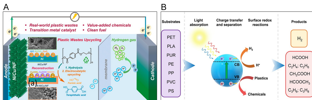
Figure 6. (A) Upcycling of plastic waste (PET) using electrocatalysts to generate hydrogen: sourced from [88] . (B) Schematic of photoreforming pathways converting plastic-derived intermediates into fuels and chemicals: sourced from study [92] , Reproduced with permission, Copyright 2023, Elsevier (B).
