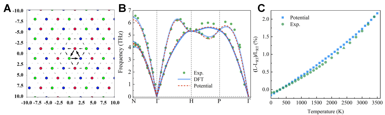
Figure 9. Validation of the machine-learned tungsten potential for dislocation core properties, lattice dynamics, and thermal behavior. (A) The core structure of a 1/2\langle 111 \rangle screw dislocation predicted by the potential shows a non-degenerate compact configuration. The different colors of the atoms (red, green, and blue) denote three consecutive (111) atomic planes along the dislocation line; (B) Comparison of phonon dispersion curves with experimental measurements and DFT calculations; (C) Comparison of the change in the thermal expansion coefficient with temperature and experimental data. DFT: Density functional theory.
