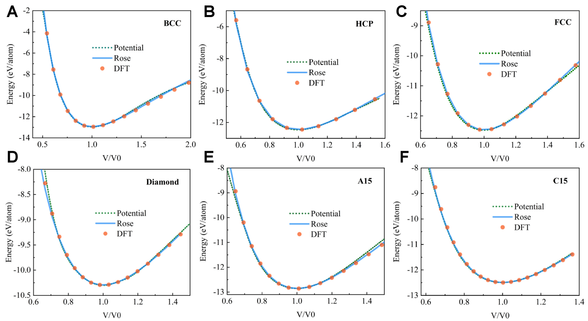
Figure 2. Comparison of the E-V relationships for various pure tungsten polymorphs calculated using the Rose EOS, first-principles DFT calculations, and trained MLP (called “Potential” in the figure). The horizontal axes represent the relative volume ( V/V_0 ), and the vertical axes represent the energy per atom (eV/atom), illustrating the structural stability under isotropic deformation. (A) BCC ground-state structure; (B) HCP structure; (C) FCC structure; (D) Diamond structure; (E) A15 structure; (F) C15 structure. E-V: Energy-volume; EOS: equation of state; DFT: density functional theory; MLP: machine-learning potential; BCC: body-centered cubic; HCP: hexagonal close-packed; FCC: face-centered cubic.
