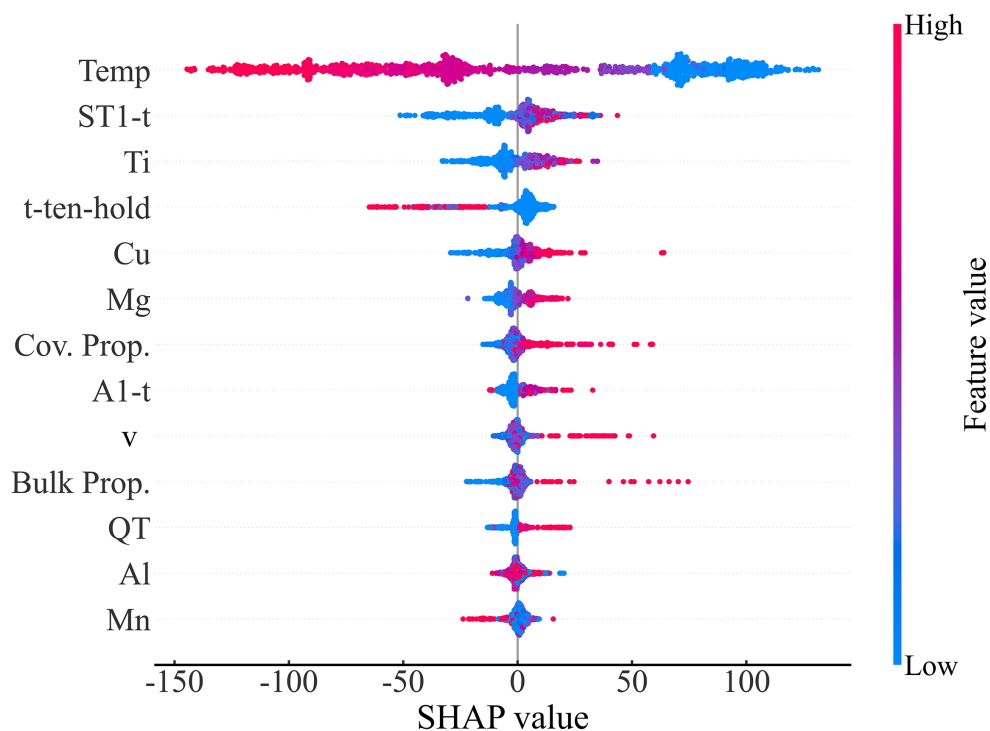
Figure 9. SHAP bee swarm plot (summary plot) obtained from the trained RF model. Each dot represents a sample in the dataset. The horizontal axis represents the corresponding SHAP value of the feature, where positive and negative values indicate positive and negative contributions to the UTS, respectively, and the absolute value reflects the magnitude of the contribution. The color of the dots represents the normalized feature value (blue for low values, red for high values). Features are ranked from top to bottom according to their mean absolute SHAP values (mean|SHAP|). SHAP: SHapley Additive exPlanations; RF: random forest; UTS: ultimate tensile strength.
