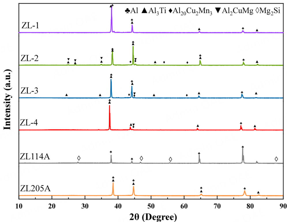
Figure 6. XRD patterns of the investigated alloys. XRD: X-ray diffraction.
