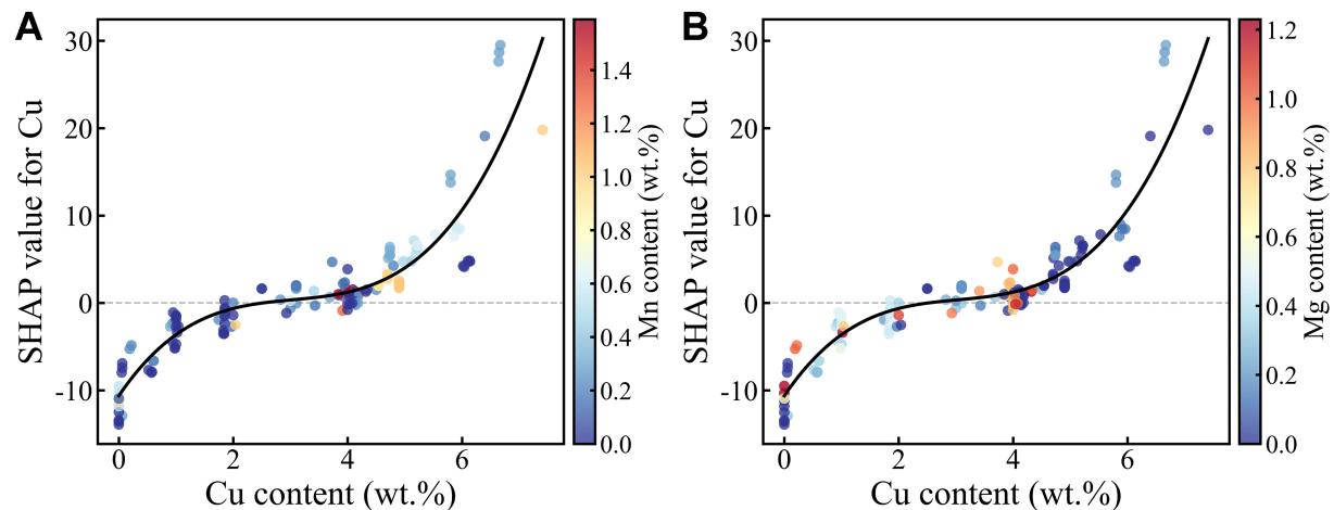
Figure 10. SHAP dependence plots for Cu content. (A) Colored by Mn content; (B) Colored by Mg content. The black fitted curve represents the overall trend between the Cu content and its SHAP value, while the color of the scatter points reflects the relative concentration of the corresponding modulating elements. SHAP: SHapley Additive exPlanations.
