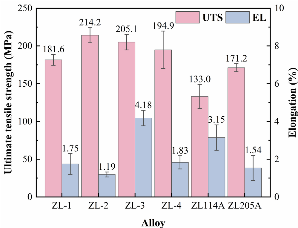
Figure 5. Elevated-temperature UTS and elongation of the investigated alloys tested at 300 °C. The data are presented as the mean \pm SD of three replicate tensile tests for each alloy ( n = 3 ). UTS: Ultimate tensile strength; SD: standard deviation; EL: elongation.
