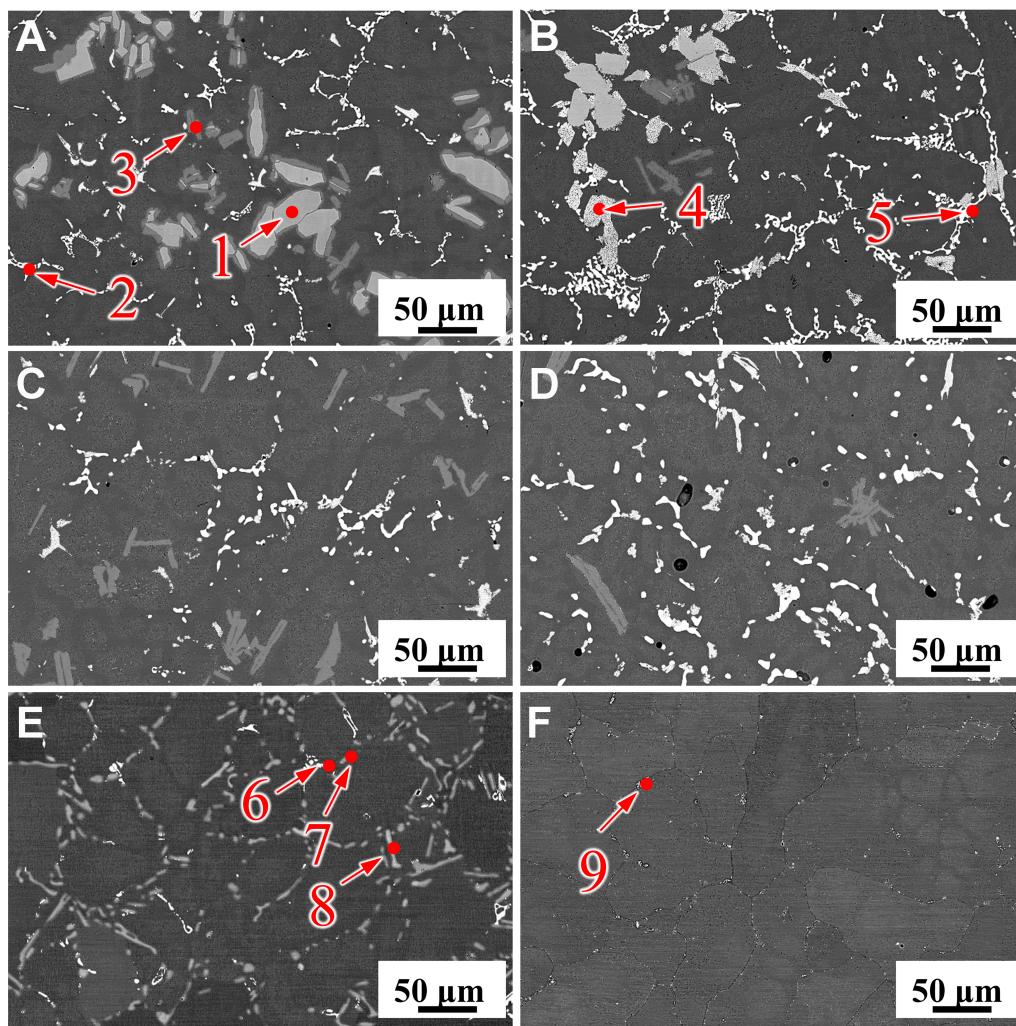
Figure 7. The microstructures of the alloys are as follows: (A) ZL-1, (B) ZL-2, (C) ZL-3, (D) ZL-4, (E) ZL114A, (F) ZL205A.
