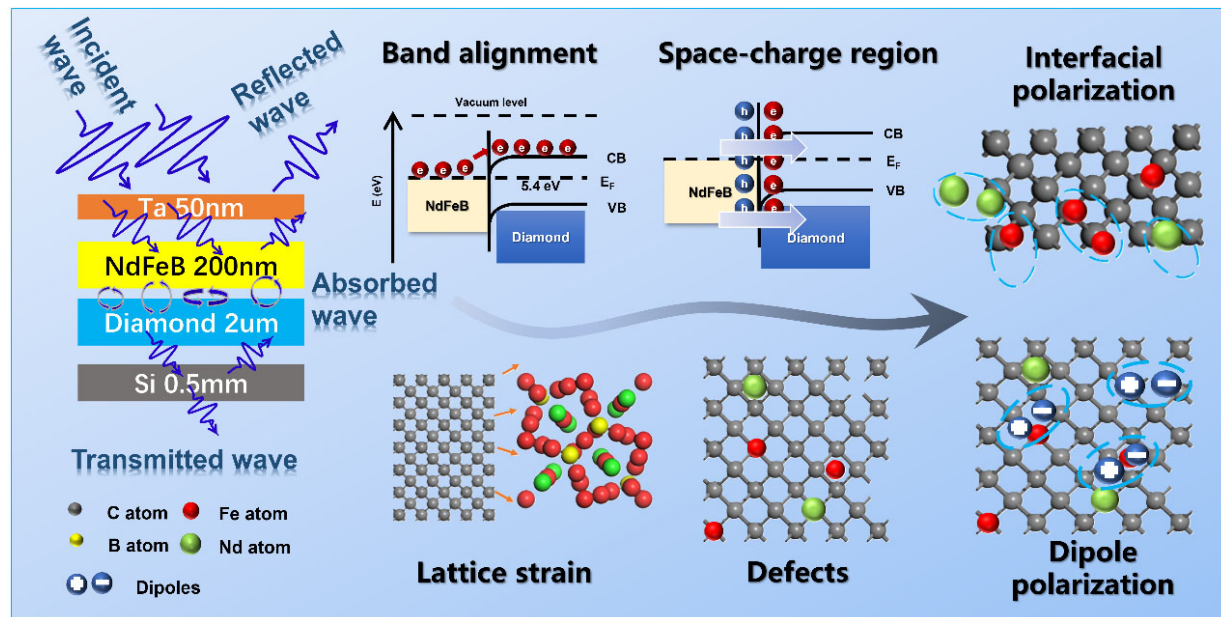
Figure 6. Schematic illustrations for the TEMW absorption mechanism of SDNT2 sample. TEMW: Terahertz electromagnetic waves; CB: conduction band; VB: valence band; E_F : Fermi level; SDNT: Si/diamond/NdFeB/Ta.
