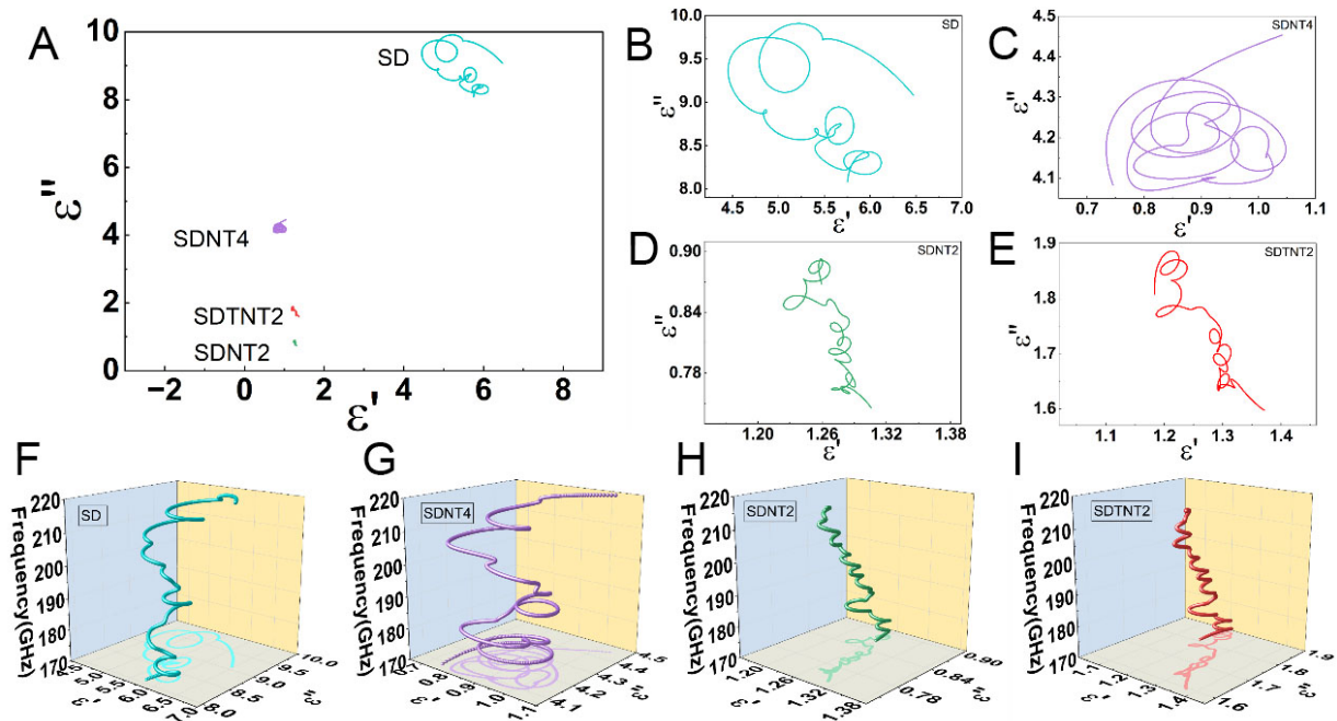
Figure 5. Cole-Cole plots of diamond/NdFeB composite films in the 170–220 GHz range. (A) overall plot, (B and F) 2D and 3D Cole-Cole plots for the SD sample, respectively; (C and G) 2D and 3D Cole-Cole plots for the SDNT4 sample, respectively; (D and H) 2D and 3D Cole-Cole plots for the SDNT2 sample, respectively; (E and I) 2D and 3D Cole-Cole plots for the SDTNT2 sample, respectively. SD: Si/diamond; SDNT: Si/diamond/NFB/Ta; SDTNT: Si/diamond/Ta/NFB/Ta.
