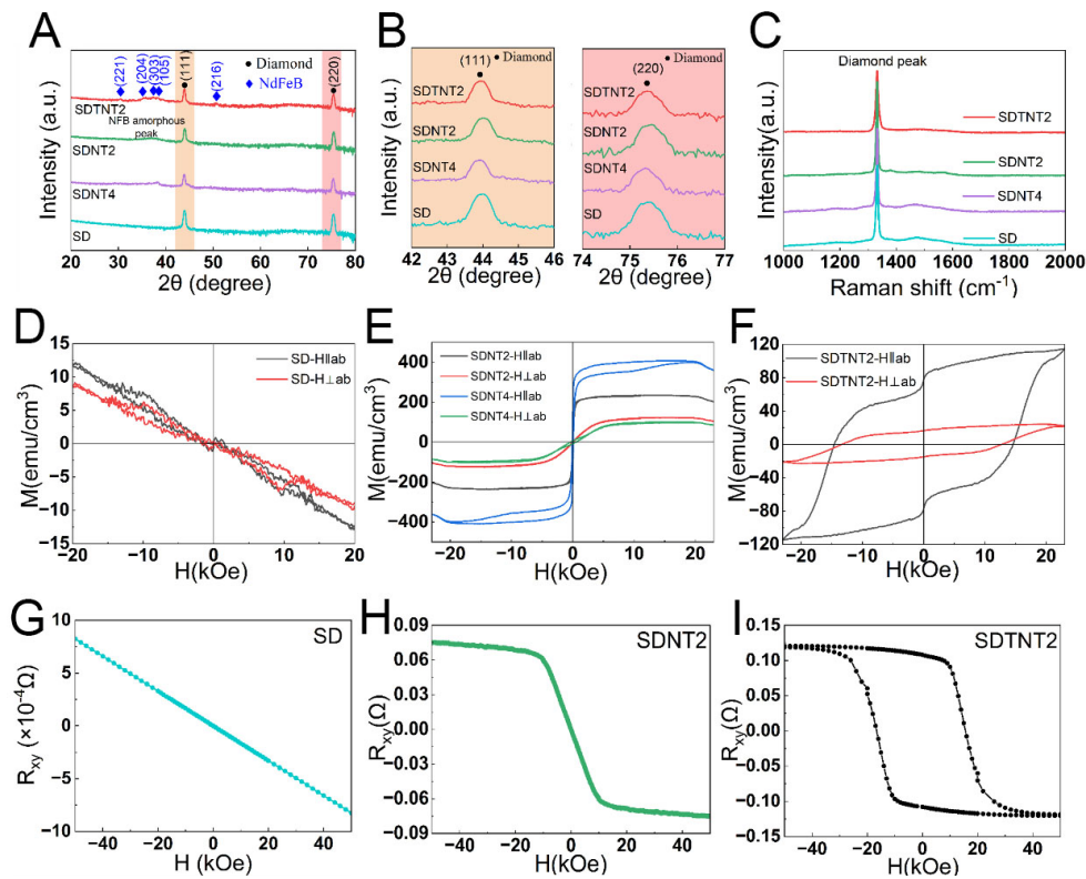
Figure 1. Structure and electromagnetic properties of diamond/NdFeB composite films. (A) GIXRD spectra, (B) magnified XRD spectra of diamond (111) and (220) crystal planes, (C) Raman spectra in the range of 1,000–2,000 \text{cm}^{-1} , Room temperature M - H hysteresis loop of (D) SD, (E) SDNT2 and SDNT4, (F) SDTNT2, Room temperature Hall resistance curve of (G) SD, (H) SDNT2, (I) SDTNT2. SDTNT: Si/diamond/Ta/NFB/Ta; SDNT: Si/diamond/NFB/Ta; SD: Si/diamond; GIXRD: grazing-incidence X-ray diffraction.
