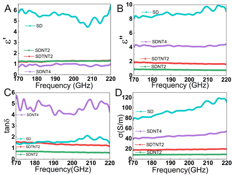
Figure 4. Dielectric properties of diamond/NdFeB composite thin films in the frequency range of 170–220 GHz: (A) real part of dielectric constant; (B) imaginary part of dielectric constant; (C) loss tangent, (D) electrical conductivity.
