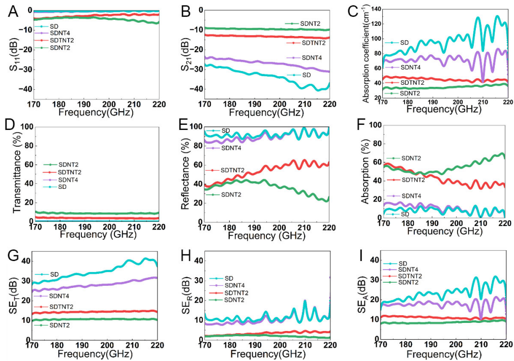
Figure 3. Electromagnetic wave absorption properties of diamond/NdFeB composite films in the frequency range of 170–220 GHz. (A) S_{11} parameter, (B) S_{21} parameter, (C) absorption coefficient, (D) transmittance, (E) reflectance, (F) absorptivity, (G) total EMI SE, (H) reflection EMI SE, (I) absorption EMI SE. SD: Si/diamond; SDNT: Si/diamond/NdFeB/Ta; SDTNT: Si/diamond/Ta/NdFeB/Ta; EMI: electromagnetic interference; SE: shielding effectiveness.
