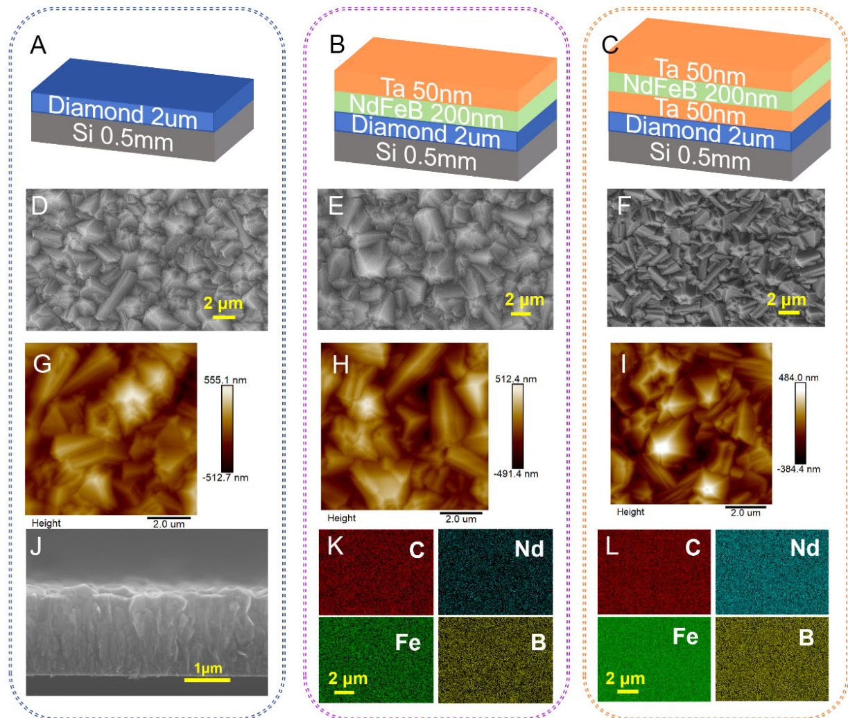
Figure 2. Morphology and elemental analysis characterization of diamond/NdFeB composite films. (A–C) Schematic diagrams of film growth for SD, SDNT2 and SDTNT2 samples, (D–F) Surface SEM of the corresponding samples, (G–I) AFM of the corresponding samples, (J) Cross-sectional SEM of the SD sample, (K and L) EDS elemental analysis of SDNT2 and SDTNT2 samples. SD: Si/diamond; SDNT: Si/diamond/NdFeB/Ta; SDTNT: Si/diamond/Ta/NdFeB/Ta; SEM: scanning electron microscope; AFM: atomic force microscope; EDS: energy-dispersive X-ray spectroscopy.
