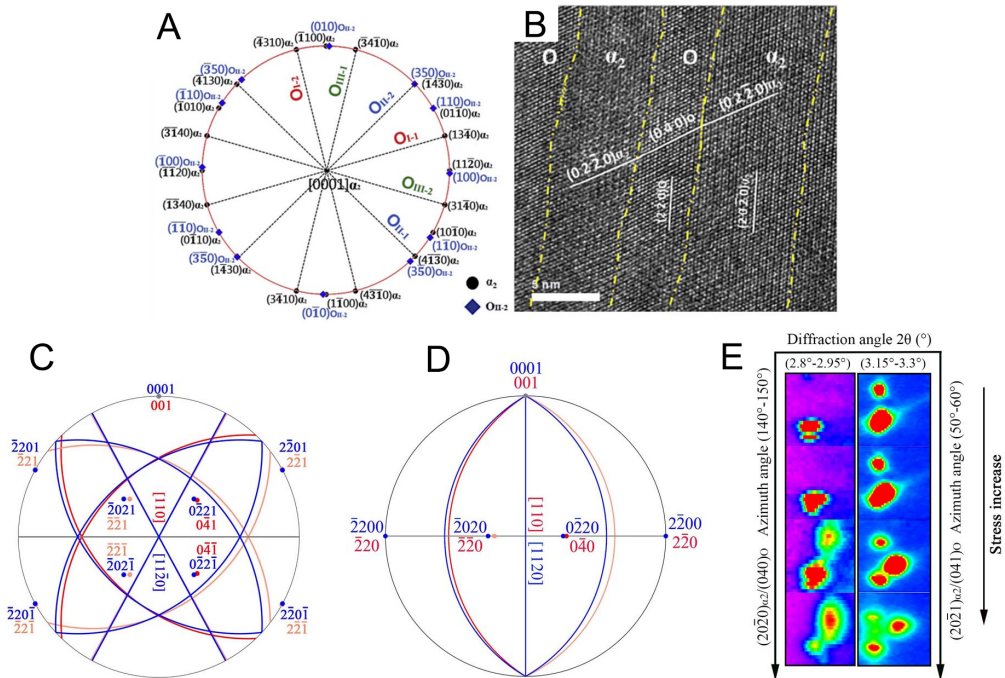
Figure 13. (A) [0001]_{\alpha_2} superimposed pole figures showing the lattice correspondence between the \alpha_2 and O phases, with the calculated habit planes being (1430)_{\alpha_2} ; (B) HRTEM image recorded along [0001]_{\alpha_2} . (Reproduced from Ref.[88] [88] ); The [11\bar{2}0]_{\alpha_2}/[110]_O superimposed pole figure exhibits the lattice correspondence of (C) equivalent \{20\bar{2}1\}_{\alpha_2} planes and \{221\}_O and \{041\}_O planes and (D) equivalent \{20\bar{2}0\}_{\alpha_2} planes and \{220\}_O and \{040\}_O planes; (E) Evolution of the (20\bar{2}0)_{\alpha_2} and (040)_O reflection doublet and (20\bar{2}1)_{\alpha_2} and (041)_O reflection doublet with increasing stress. (Reproduced from Ref.[37] [37] ). HRTEM: High-resolution transmission electron microscopy.
