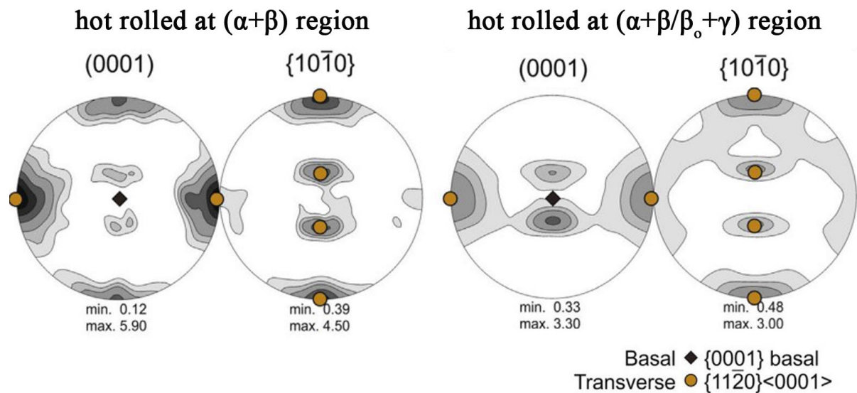
Figure 7. Pole figures of the \alpha_2 phase in a Ti-43Al-4Nb-1Mo-0.1B alloy hot rolled in different phase regions. The RD is aligned vertically, and the TD horizontally. (Reproduced from Ref.[72] [72] ). RD: Radial direction; TD: transverse direction.
