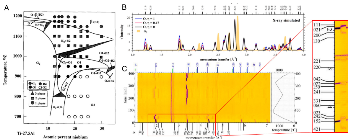
Figure 11. (A) Ternary Ti-27.5Al-xNb phase diagram. (Reproduced from Ref.[38] [38] ); (B) Simulated XRD patterns of the O phase with the chemical composition of Ti 2 AlNb; (C) Variation of the Ti-24.8Al-24.3Nb neutron diffraction pattern at different temperatures. (Reproduced from Ref.[90] [90] ). XRD: X-ray diffraction.
