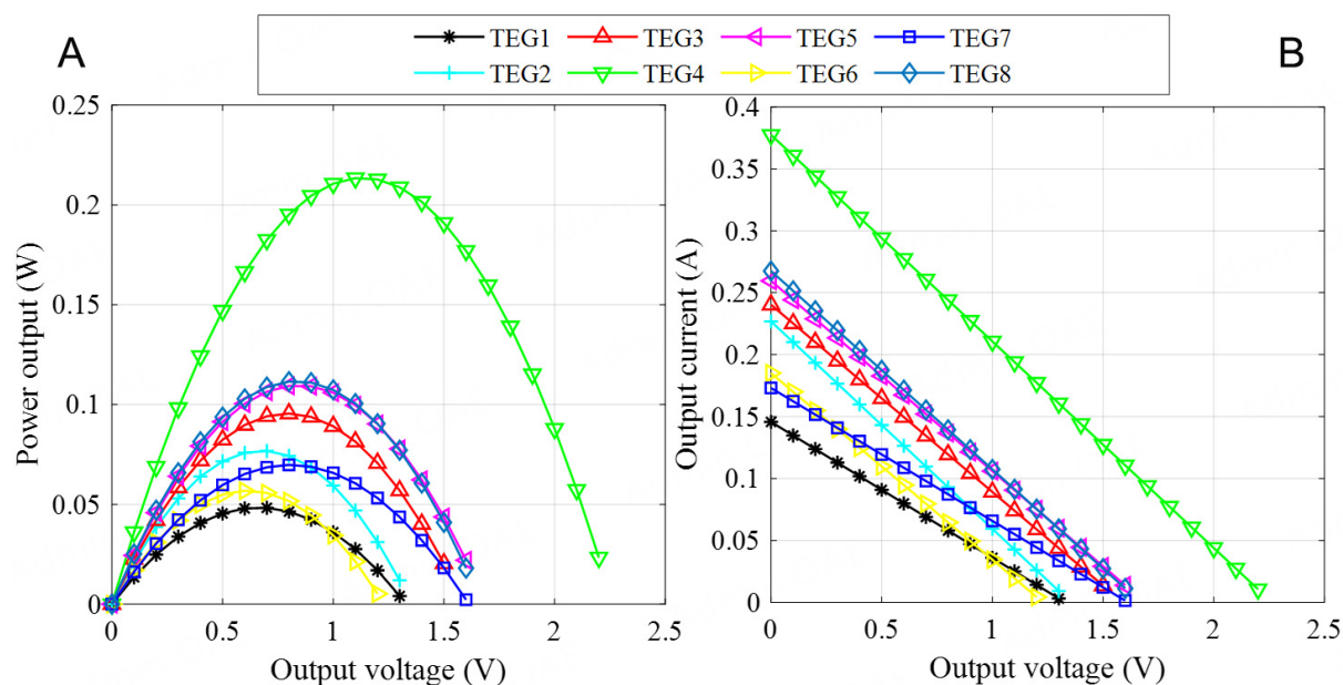
Figure 4. Electrical output of the different TEG modules (A) Power-voltage, (B) Current-voltage profiles.
