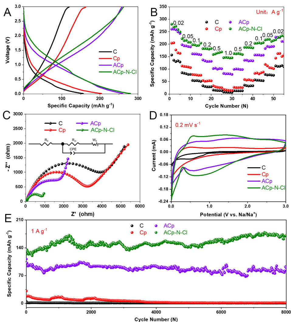
Figure 4. (A) Charge-discharge curves, (B) multiplication rate performance, (C) EIS spectra, (D) CV curves and (E) stability test at 1 A g -1 of C, Cp, ACp and ACp-N-Cl. EIS: Electrochemical impedance spectroscopy; CV: cyclic voltammetry.
