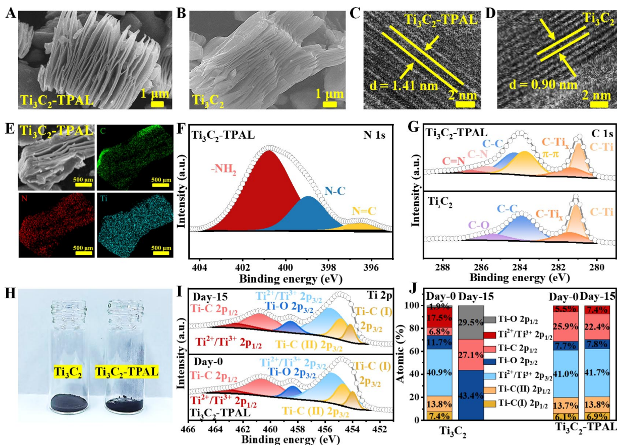
Figure 2. SEM images of (A) \text{Ti}_3\text{C}_2 -TPAL and (B) \text{Ti}_3\text{C}_2 . HRTEM images of (C) \text{Ti}_3\text{C}_2 -TPAL and (D) \text{Ti}_3\text{C}_2 . (E) SEM image and elemental mappings of \text{Ti}_3\text{C}_2 -TPAL. High-resolution XPS spectra of \text{Ti}_3\text{C}_2 -TPAL in the (F) N 1s and (G) C 1s regions. (H) Digital photographs of \text{Ti}_3\text{C}_2 and \text{Ti}_3\text{C}_2 -TPAL after aging under ambient conditions. (I) Fitted Ti 2p XPS spectra and (J) relative atomic percentages of Ti species derived from Ti 2p fitting for \text{Ti}_3\text{C}_2 and \text{Ti}_3\text{C}_2 -TPAL before and after aging.
