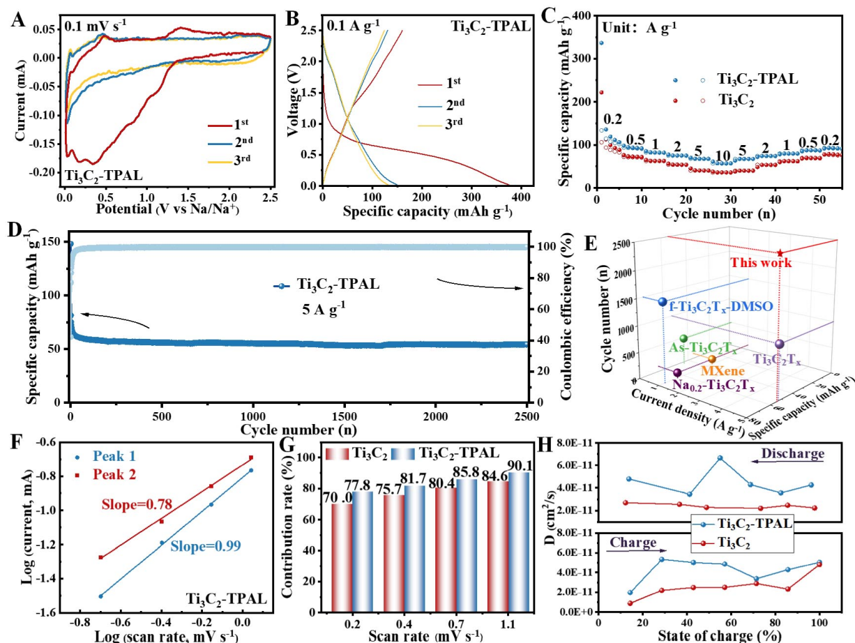
Figure 3. (A) CV curves recorded at a scan rate of 0.1 mV s -1 , (B) galvanostatic charge-discharge plots tested at 0.1 A g -1 , (C) rate capability under different current densities, and (D) long-cycle durability at 5 A g -1 of Ti 3 C 2 -TPAL. (E) Performance comparison with previously reported MXene-based anodes. (F) Relationship between peak current and scan rate of Ti 3 C 2 -TPAL. (G) Capacitive contribution fractions and (H) Na + diffusion coefficients of Ti 3 C 2 -TPAL and Ti 3 C 2 .
