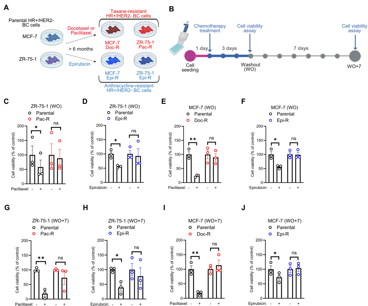
Figure 1. Drug response profiling validates stable chemoresistant phenotypes in HR+/HER2- BC models. (A) Schematic representation of the generation of anthracycline- and taxane-resistant cell populations from parental HR+/HER2- BC cell lines (MCF-7 and ZR-75-1). Created in BioRender. Corbet, C. (2026) https://BioRender.com/i5zflea ; (B) Experimental design of the drug challenge and recovery assays. Cells were treated with chemotherapeutic agents for 72 h, followed by drug WO and a 7-day recovery period (WO+7). Created in BioRender. Corbet, C. (2026) https://BioRender.com/eoukvmv ; (C and D) Viability of parental and drug-resistant ZR-75-1 cells after 72 h of treatment (WO) with 25 nM paclitaxel (C) or 10 nM epirubicin (D); (E and F) Viability of parental and drug-resistant MCF-7 cells after 72 h of treatment (WO) with 25 nM paclitaxel (E) or 30 nM epirubicin (F); (G and H) Viability of parental and drug-resistant ZR-75-1 cells following 72 h of treatment with 25 nM paclitaxel (G) or 10 nM epirubicin (H), and subsequent culture in drug-free medium for 7 days (WO+7); (I and J) Viability of parental and drug-resistant MCF-7 cells following 72 h of treatment with 25 nM paclitaxel (I) or 30 nM epirubicin (J), and subsequent culture in drug-free medium for 7 days (WO+7). Data are presented as mean \pm SEM from three independent biological experiments ( n = 3 ), each performed with three technical replicate wells per condition (C-J). Individual data points represent the mean of the technical replicates from each independent biological experiment. Statistical significance was determined using two-way ANOVA with Sidák's multiple comparison test (C-J). * P < 0.05 ; ** P < 0.01 ; ns: not significant. HR+/HER2-: Hormone receptor-positive/human epidermal growth factor receptor 2-negative; BC: breast cancer; WO: washout; SEM: standard error of the mean; ANOVA: analysis of variance; Doc-R: docetaxel-resistant; Pac-R: paclitaxel-resistant; Epi-R: epirubicin-resistant.
