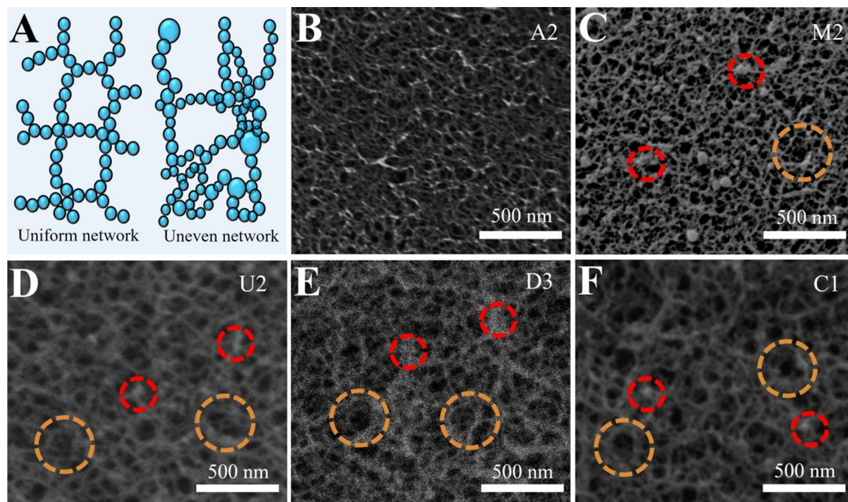
Figure 3. Network structure of aerogel film samples. (A) Diagrams of a uniform network and an uneven network; (B-F) SEM micrographs of silica aerogel films. The red circle represents typical agglomerated particles, and the orange areas represent typically large holes that facilitate gas diffusion. SEM: Scanning electron microscopy.
