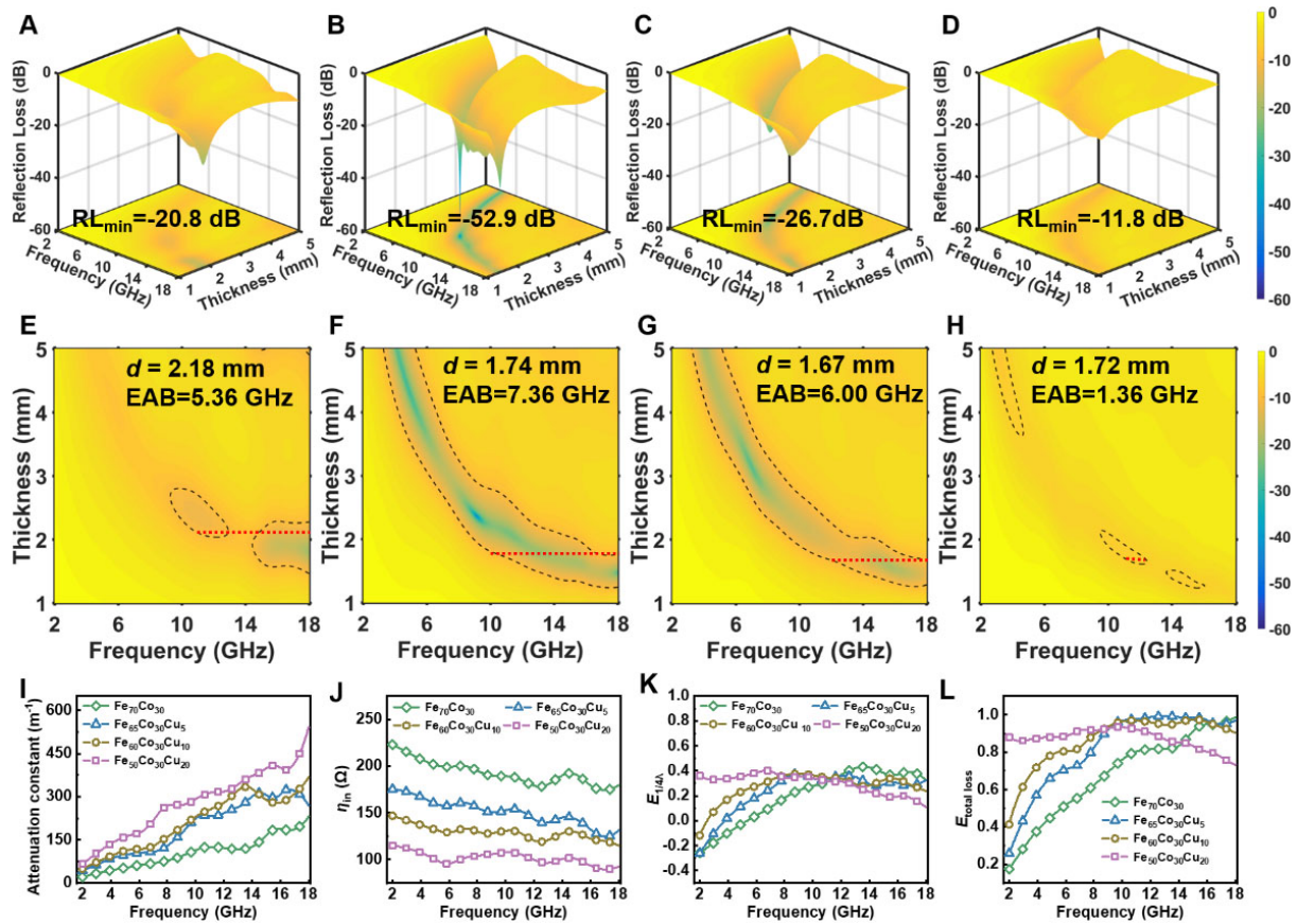
Figure 5. EM wave absorption performance and loss mechanism analysis of FeCoCu alloy foams with different Cu contents. Three-dimensional reflection loss maps of (A) \text{Fe}_{70}\text{Co}_{30} , (B) \text{Fe}_{65}\text{Co}_{30}\text{Cu}_5 , (C) \text{Fe}_{60}\text{Co}_{30}\text{Cu}_{10} and (D) \text{Fe}_{50}\text{Co}_{30}\text{Cu}_{20} , respectively. Corresponding two-dimensional reflection loss contour maps of (E) \text{Fe}_{70}\text{Co}_{30} , (F) \text{Fe}_{65}\text{Co}_{30}\text{Cu}_5 , (G) \text{Fe}_{60}\text{Co}_{30}\text{Cu}_{10} and (H) \text{Fe}_{50}\text{Co}_{30}\text{Cu}_{20} , respectively. The dashed contour lines indicate \text{RL} = -10 dB, and the maximum EABs are marked in the corresponding panels. Frequency-dependent (I) attenuation constant, (J) input impedance, (K) interference loss contribution, and (L) total energy loss contribution are presented to clarify the EM absorption mechanism. EM: Electromagnetic; RL: reflection loss; EAB: effective absorption bandwidth.
