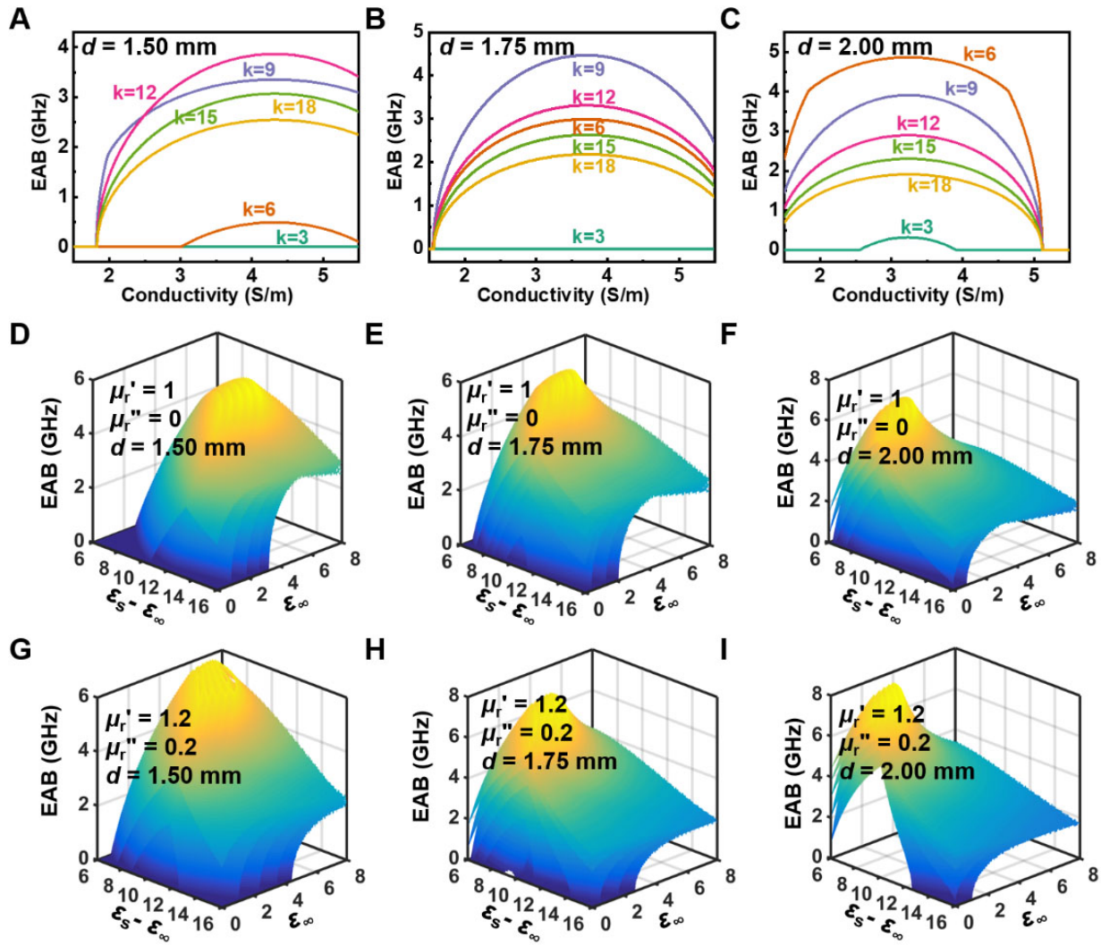
Figure 2. EAB maps of conduction-loss-dominated EWAMs as functions of electrical conductivity \sigma and the constant real permittivity k ( \epsilon_r' = k ) with coating thicknesses of (A) 1.50, (B) 1.75, and (C) 2.00 mm, respectively. Three-dimensional maps of EABs as a function of \epsilon_\infty , \epsilon_s , and \tau for polarization-loss-dominated materials with coating thicknesses of (D) 1.50, (E) 1.75, and (F) 2.00 mm, respectively. Corresponding EAB distributions after introducing magnetic loss ( \mu_r' = 1.2 and \mu_r'' = 0.2 ) with coating thicknesses of (G) 1.50, (H) 1.75, and (I) 2.00 mm, respectively. EAB: Effective absorption bandwidth; EWAM: electromagnetic wave absorbing material.
