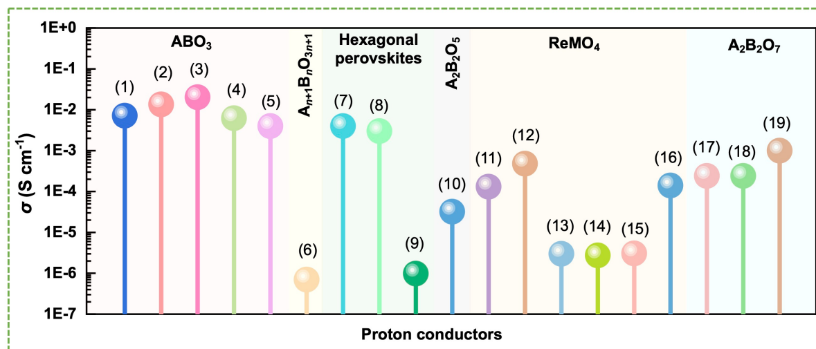
Figure 5. Total conductivity of proton conductors at 500 °C. Abbreviations: (1) BaZr_{0.1}Ce_{0.7}Y_{0.2}O_{3-\delta} , BZCY172 [45] ; (2) BZCYYb1711 [45] ; (3) BZCYYb4411 [47] ; (4) BZCYYb4411 [53] ; (5) BaSc_{0.8}Mo_{0.2}O_{2.8} [48] ; (6) BaLaInO_4 [50] ; (7) Ba_7Nb_4MoO_{20} [54] ; (8) Ba_5Er_2Al_2ZrO_{13} [51] ; (9) \gamma - Ba_4Ta_2O_9 [55] ; (10) Ba_2In_2O_5 [49] ; (11) La_{0.99}Ca_{0.01}NbO_4 [56] ; (12) La_{0.99}Ca_{0.01}TaO_4 [52] ; (13) Nd_{0.99}Ca_{0.01}TaO_4 [52] ; (14) Gd_{0.99}Ca_{0.01}TaO_4 [52] ; (15) Er_{0.99}Ca_{0.01}TaO_4 [52] ; (16) La_{0.8}Ba_{1.2}GaO_{3.9} [49] ; (17) La_{1.95}Ca_{0.05}Zr_2O_7 [49] ; (18) La_2Ce_2O_7 [49] ; (19) La_{1.95}Ca_{0.05}Ce_2O_7 [57] .
