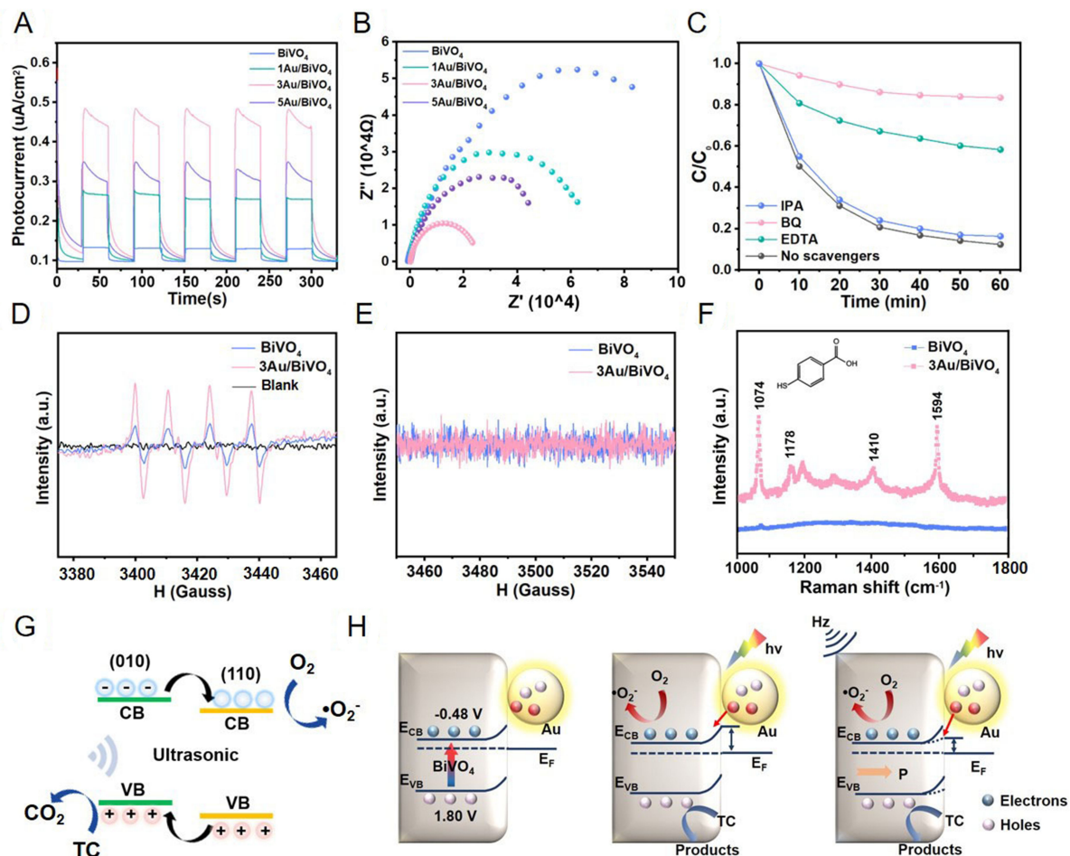
Figure 6. (A) The transient photocurrent response curves of \text{BiVO}_4 and \text{Au/BiVO}_4 catalysts; (B) EIS plots of \text{BiVO}_4 and \text{Au/BiVO}_4 catalysts; (C) Active species capture experiments in piezo-photocatalytic processes; ESR spectra of (D) \text{DMPO-O}_2^{\bullet-} and (E) \text{DMPO}\cdot\text{OH} ; (F) Surface enhanced Raman scattering testing of 4-MBA on the \text{BiVO}_4 and 3\text{Au/BiVO}_4 heterostructure; (G) Schematic illustration for (010) and (110) surface heterojunction; (H) Schematic diagram of piezo-/photocatalytic mechanism. \text{BiVO}_4 : Bismuth vanadate; EIS: electrochemical impedance spectroscopy; ESR: electron spin resonance; DMPO: 5,5-dimethyl-1-pyrroline N-oxide; 4-MBA: 4-mercaptobenzoic acid.
