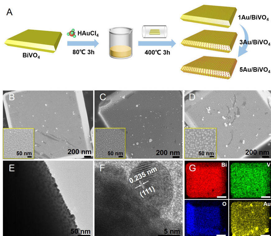
Figure 1. (A) Schematic diagram of the synthesis route of the x\text{Au}/\text{BiVO}_4 heterojunction; (B-D) SEM images of the x\text{Au}/\text{BiVO}_4 heterostructures ( x = 1, 3, 5 ); (E and F) HRTEM images of 3\text{Au}/\text{BiVO}_4 ; (G) EDS elemental mapping images of the 3\text{Au}/\text{BiVO}_4 heterostructures. The scales in Figure 1G all represent 1 \mu\text{m} . \text{BiVO}_4 : Bismuth vanadate; SEM: scanning electron microscope; HRTEM: high-resolution transmission electron microscopy; EDS: energy-dispersive X-ray spectroscopy.
