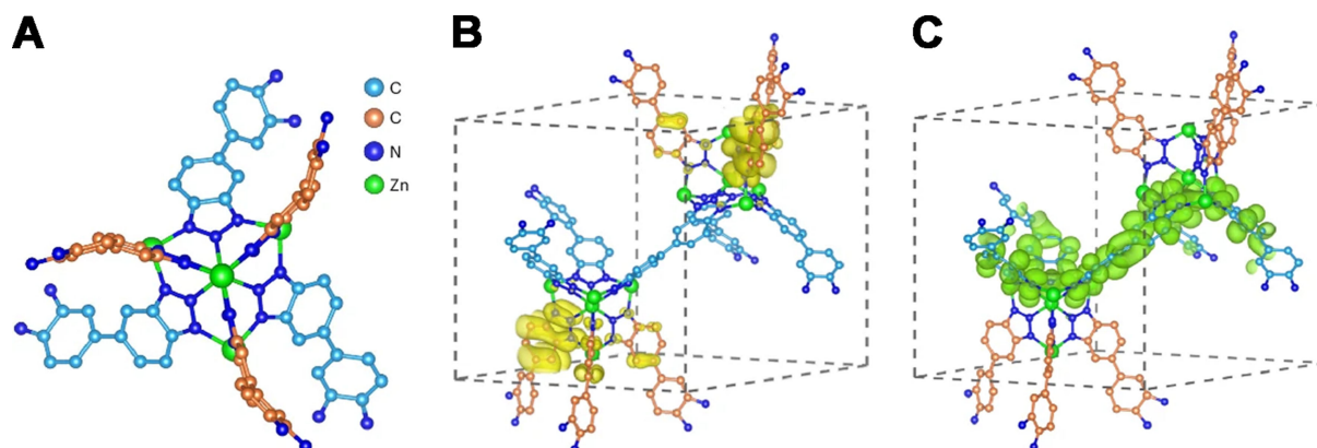
Figure 1. (A) The secondary building unit in CFA-Zn with hydrogen atoms and acetate omitted. The orange and light blue benzene rings represent crystallographically different ligands; (B and C) Spatial distribution of the (B) VBM and (C) CBM of the ground state in the MOF single cell with the isosurface value of 0.003 e \text{ \AA}^{-3} . The yellow bubbles and green bubbles represent the electron clouds [10] . CFA-Zn: Coordination Framework Augsburg-Zn; VBM: valence band maximum; CBM: conduction band minimum; MOF: metal-organic framework.
