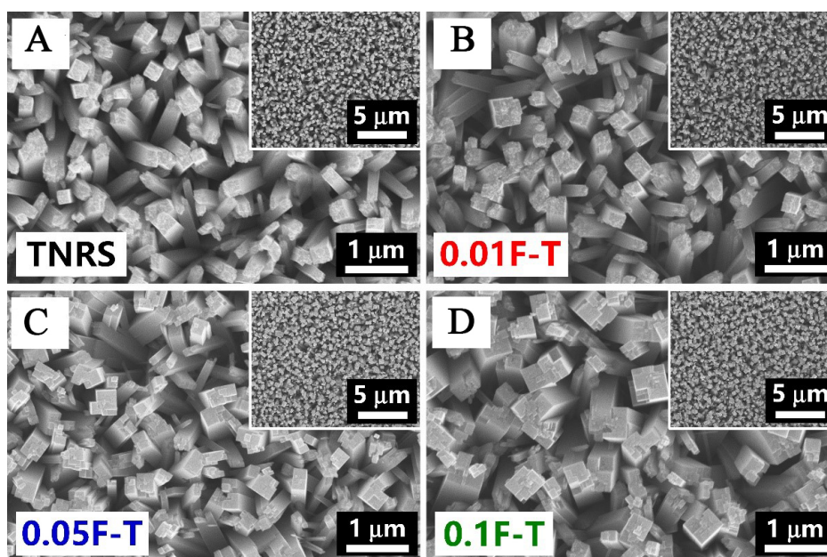
Figure 2. SEM images of (A) pristine TNRS photoanode; (B) 0.01F-T photoanode; (C) 0.05F-T photoanode; and (D) 0.1F-T. SEM: Scanning electron microscopy; TNRS: \text{TiO}_2 nanorod sample; F-T: F-doped \text{TiO}_2 nanorods.
