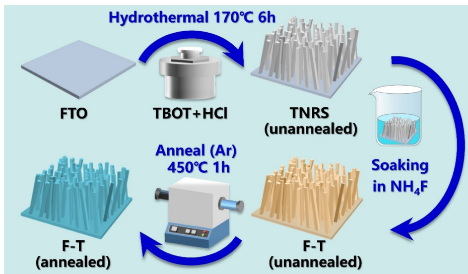
Figure 1. The typical preparation process of the F-T photoanode. TBOT: Tetrabutyl titanate; TNRS: \text{TiO}_2 nanorod sample; FTO: fluorine-doped tin oxide; F-T: F-doped \text{TiO}_2 nanorods.
