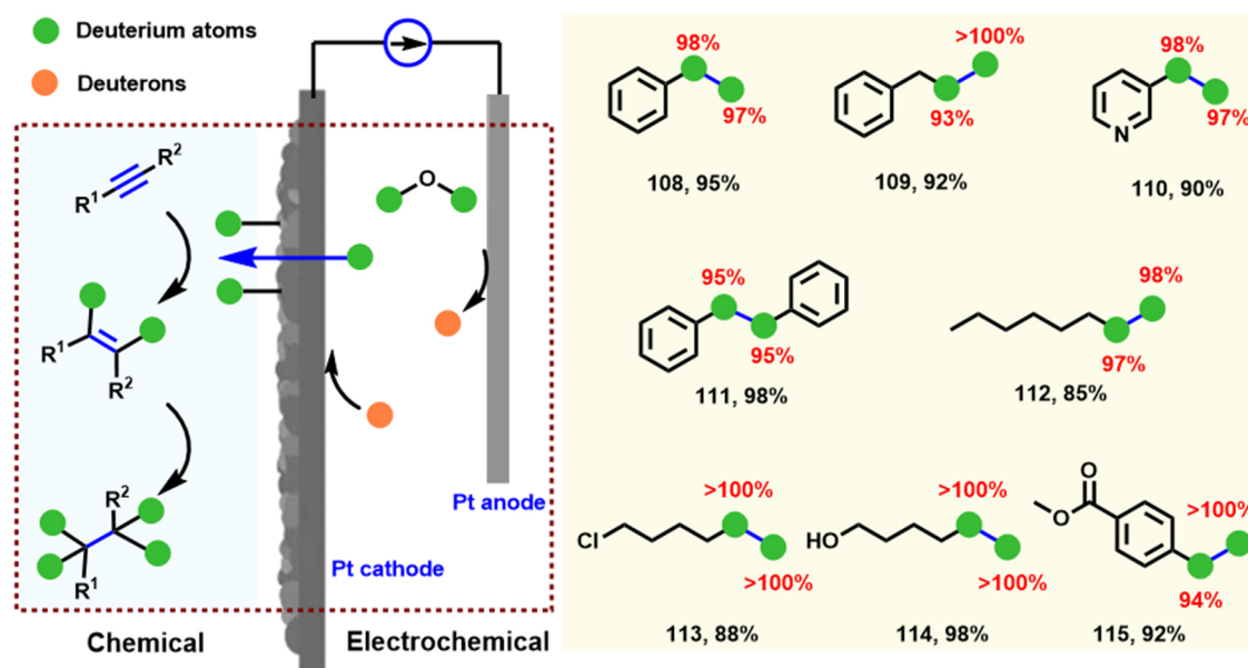
Scheme 10. Deuterium incorporation and yield by palladium membrane deuteration of alkynes. Copyright 2018, Springer Nature [78] . Red numbers: Content of 100% indicates one D atom on one carbon of products.
