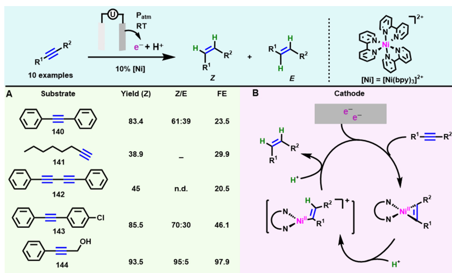
Scheme 12. Electrocatalytic semihydrogenation of alkynes with [\text{Ni}(\text{bpy})_3]^{2+} . (A) Substrate scope; (B) The formation of a nickelacyclopropene complex and Ni(II)-vinyl intermediate. Copyright 2022, American Chemical Society [83] .
