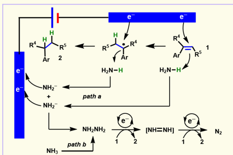
Scheme 5. Electrochemical hydrogenation of alkenes with \text{NH}_3 . (A) The scope of substrates; (B) A possible mechanism is proposed. Copyright 2019, Wiley-VCH [62] .
