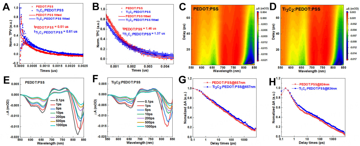
Figure 4. (A) TPV and (B) TPC for PTzBI-oF:PYF-T-o devices with and without \text{Ti}_3\text{C}_2 doping in the PEDOT:PSS interlayer; (C and D) Two-dimensional TA color plots, (E and F) TA spectra and (G and H) the trace kinetic of GSB signals of PEDOT:PSS/PTzBI-oF:PYF-T-o and \text{Ti}_3\text{C}_2 :PEDOT:PSS/PTzBI-oF:PYF-T-o bilayers. TPV: Transient photovoltage; TPC: transient photocurrent; PEDOT:PSS: poly(3,4-ethylenedioxythiophene):poly(styrenesulfonate); TA: transient absorption; GSB: ground state bleaching.
