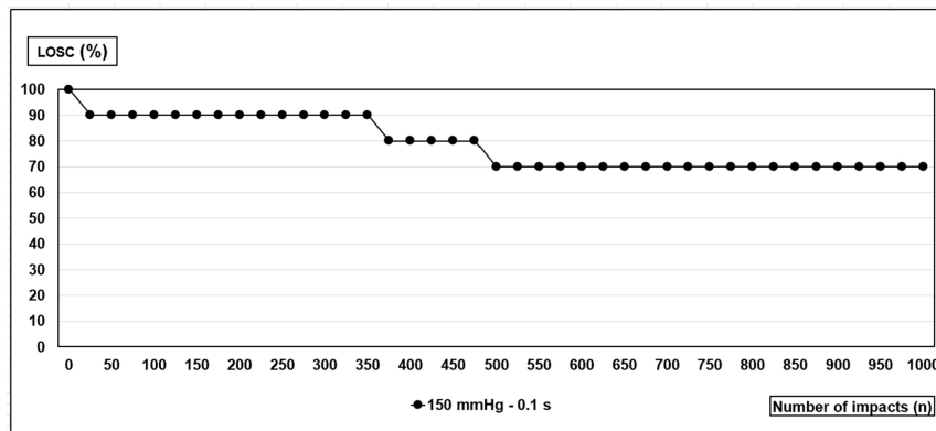
Figure 5. Likelihood of a secure closure (LOSC) until dislocation of a 15 × 15 cm mesh under a 5 cm large round defect under exposure to 1000 DIS impacts with 150 mmHg pressure peaks for 0.1 s each.
