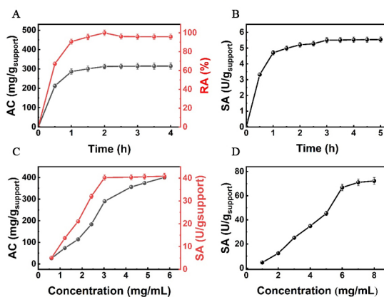
Figure 3. Effects of immobilization time on the specific activity (SA) and relative activity (RA) of immobilized enzyme and adsorption capacity (AC) of MSNs: CpsADH @MSNs (A); laccase@MSNs (B); Effects of protein concentration on the specific activity (SA) and relative activity (RA) of immobilized enzyme and adsorption capacity (AC) of MSNs: CpsADH @MSNs (C); laccase@MSNs (D).
