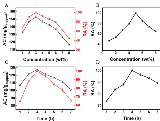
Figure 2. Effects of GA concentration on the relative activity (RA) of immobilized enzyme and adsorption capacity (AC) of MSNs: CpsADH @MSNs (A); laccase@MSNs (B); Effects of covalent bonding time on the relative activity (RA) of immobilized enzyme and adsorption capacity (AC) of MSNs: CpsADH @MSNs (C); laccase@MSNs (D).
