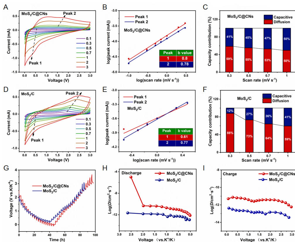
Figure 5. (A) CV curves at different scan rates from 0.1 to 3 mV s -1 for MoS 2 /C@CNs electrode. (B) Determine the value of b using the relationship between peak currents and sweep rates. (C) Calculated capacitive and diffusion-controlled contributions to the total capacity under different sweep rates. (D-F) Same CV analyses for MoS 2 /C electrode. (G) GITT voltage profiles for MoS 2 /C@CNs and MoS 2 /C electrodes. (H and I) K + diffusion coefficients calculated by GITT for MoS 2 /C@CNs and MoS 2 /C.
