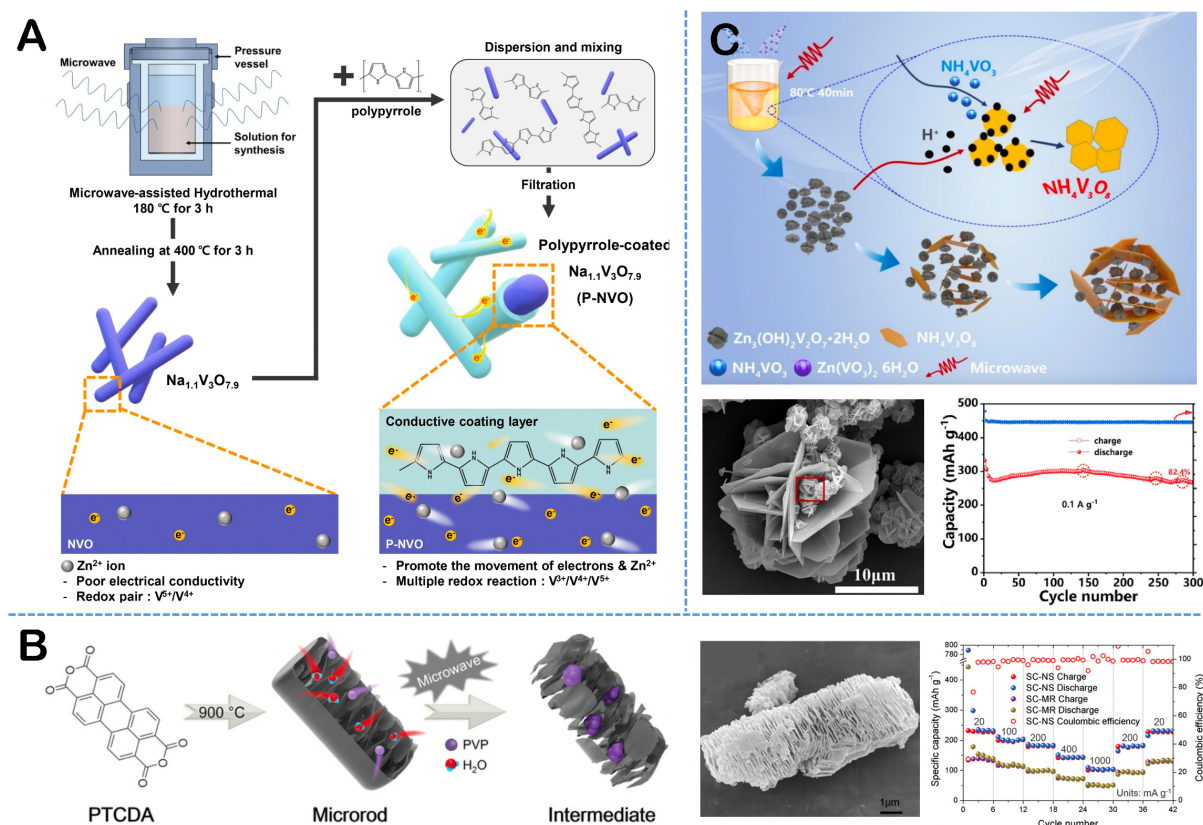
Figure 8. (A) PPy-coated \text{Na}_{1.1}\text{V}_3\text{O}_{7.9} nanorods prepared using the liquid-phase microwave method. This figure is quoted with permission [139] ; (B) Defect-rich soft carbon porous nanosheets fabricated via the liquid-phase microwave method, emphasizing their specific capacity in sodium-ion battery applications. This figure is quoted with permission [84] ; (C) 3D \text{NH}_4\text{V}_3\text{O}_8/\text{Zn}_3(\text{OH})_2\text{V}_2\text{O}_7 \cdot 2\text{H}_2\text{O} composite materials prepared using the liquid-phase microwave method, showcasing their specific capacity in zinc-ion battery applications. This figure is quoted with permission [140] .
