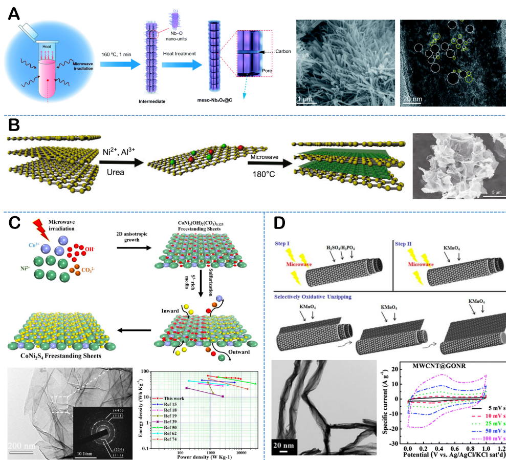
Figure 10. (A) 1D carbon-bridged \text{Nb}_2\text{O}_5 single-crystal nanorods prepared using the solid-phase microwave method. This figure is quoted with permission [148] ; (B) Ultra-large and thin NiAl layered bimetallic hydroxide nanosheets fabricated via the liquid-phase microwave method. This figure is quoted with permission [149] ; (C) Non-layered ultrathin \text{CoNi}_2\text{S}_4 nanosheets prepared using the liquid-phase microwave method, emphasizing their high energy density characteristics in supercapacitor applications. This figure is quoted with permission [60] ; (D) Nanocomposite materials MWCNT@GONR prepared through the solid-phase microwave method, focusing on their specific capacitance characteristics in supercapacitor applications. This figure is quoted with permission [150] .
