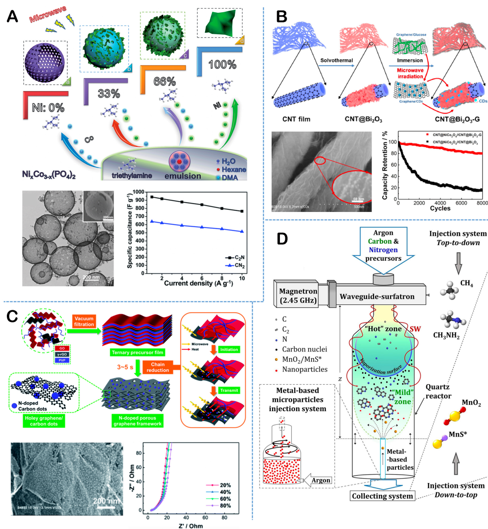
Figure 9. (A) Functionalized multi-component mesoporous Ni_xCo_{3-x}(PO_4)_2 hollow shell materials with diverse morphologies prepared via the liquid-phase microwave method, focusing on their specific capacitance characteristics in supercapacitor applications. This figure is quoted with permission [32] ; (B) Bi_2O_3 prepared on CNTs using the gas-phase microwave method, emphasizing their cycle stability in supercapacitor applications. This figure is quoted with permission [145] ; (C) OD nitrogen-doped porous graphene frameworks with nanoscale particles, fabricated using the gas-phase microwave method, showcasing their high energy density characteristics in supercapacitor applications. This figure is quoted with permission [146] ; (D) Metal oxides and metal sulfide nanoparticles prepared on nitrogen-doped graphene via the gas-phase microwave method. This figure is quoted with permission [36] .
