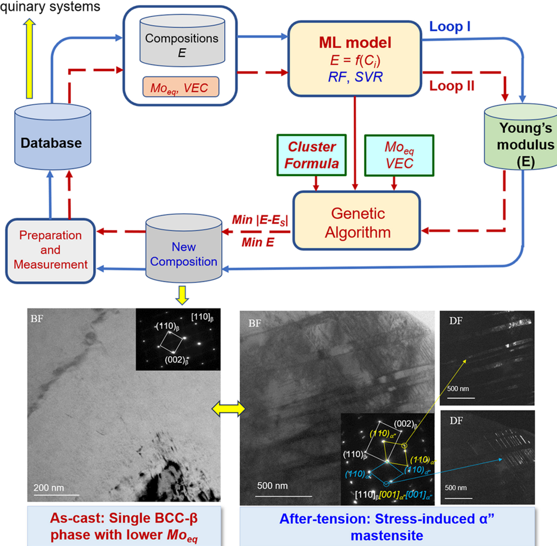
Figure 2. Cluster-formula-embedded machine learning for the design of low-E \beta -Ti alloys. The images are adapted from ref [68] with permission.
