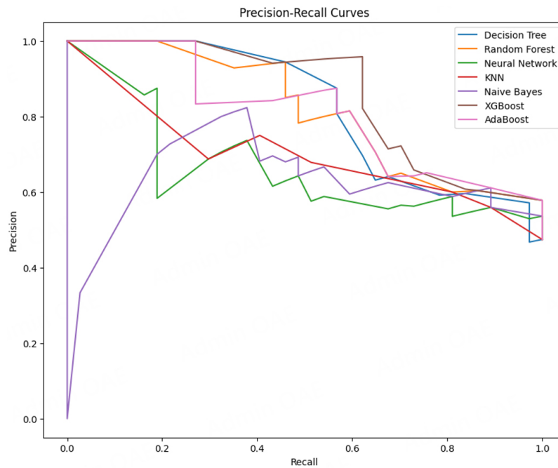
Figure 13. Precision recall curve.
