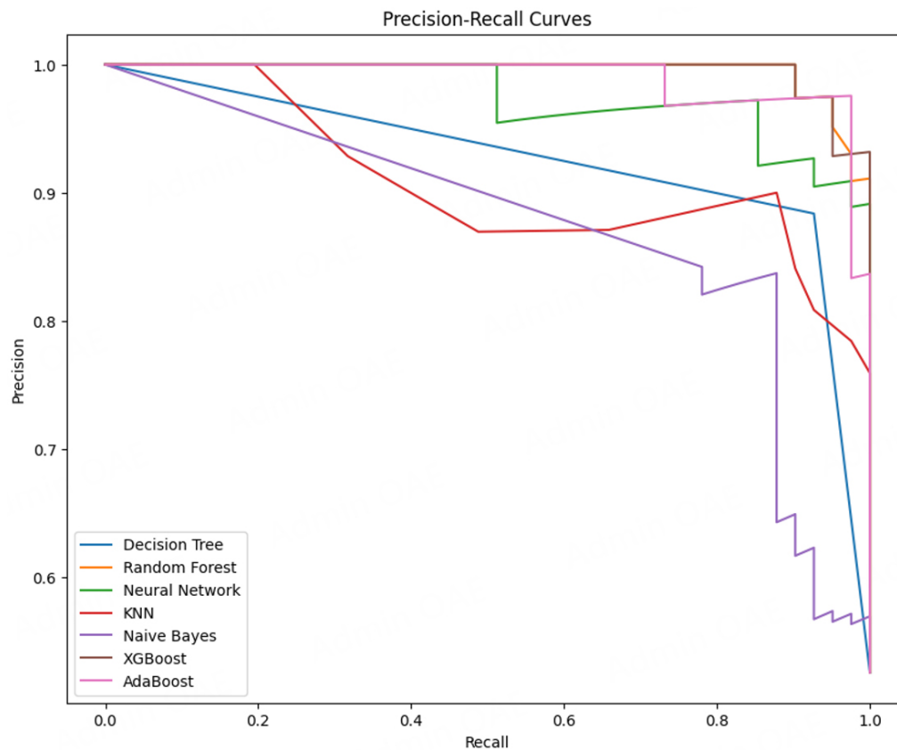
Figure 17. Precision recall curve.
