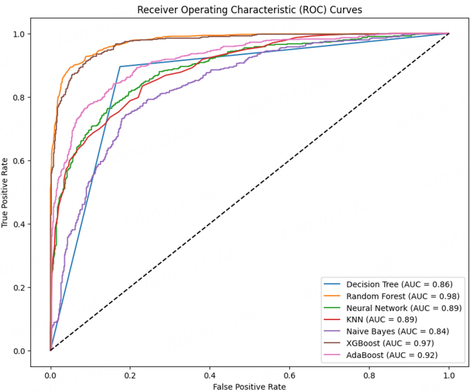
Figure 22. ROC curve.
