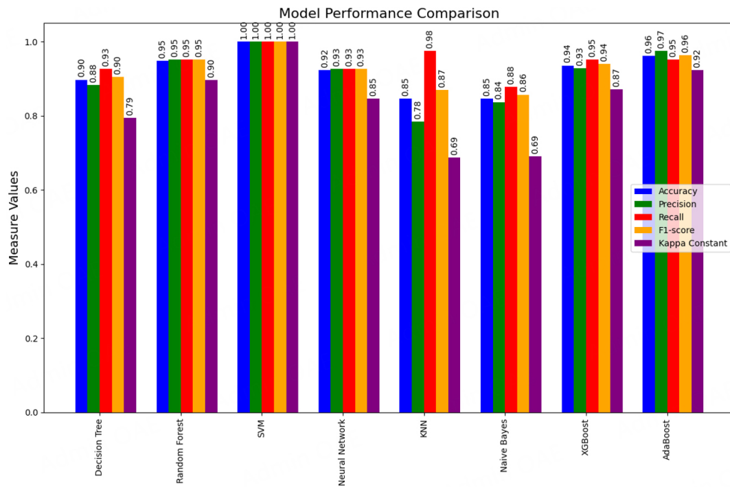
Figure 15. Performance measures.
