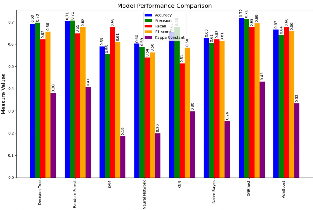
Figure 11. Performance measures.
