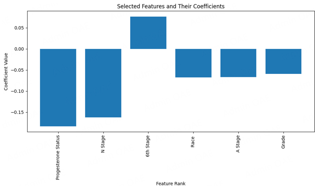
Figure 20. Selected features.
