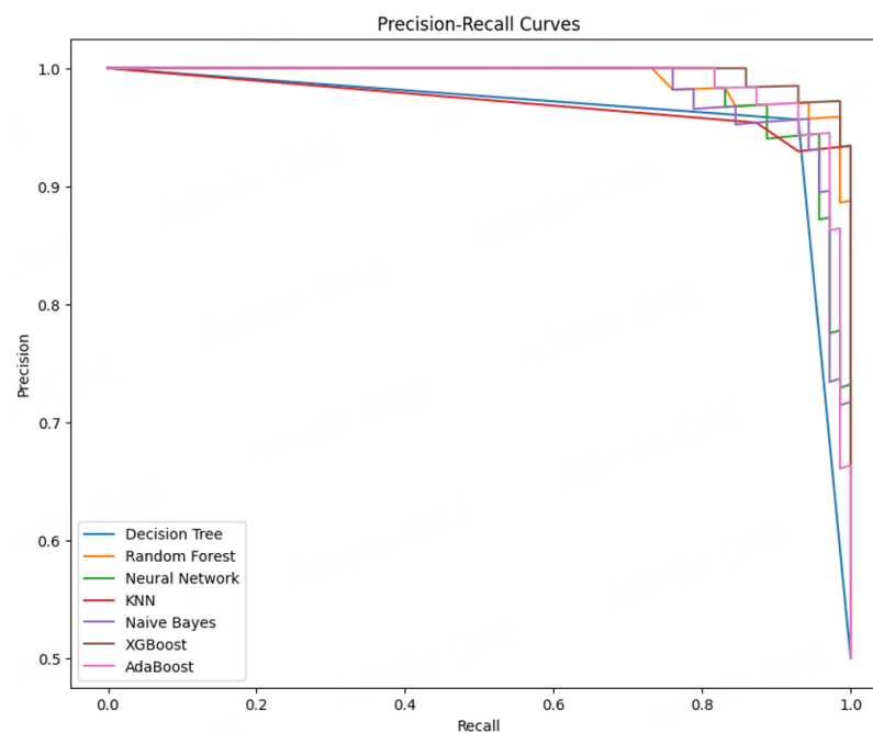
Figure 7. Precision recall curve.
