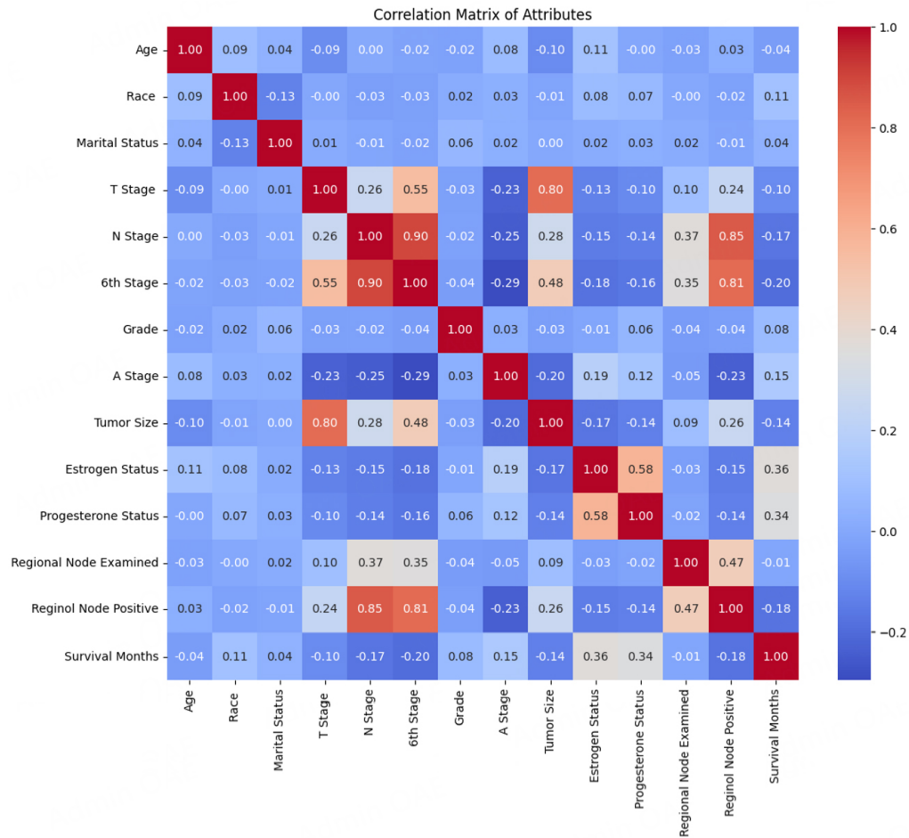
Figure 18. Correlation matrix.
