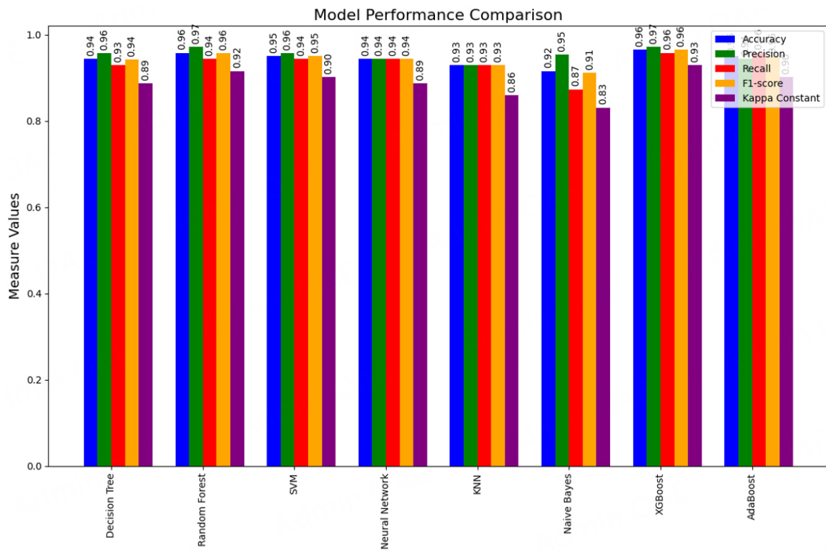
Figure 5. Performance measures.
