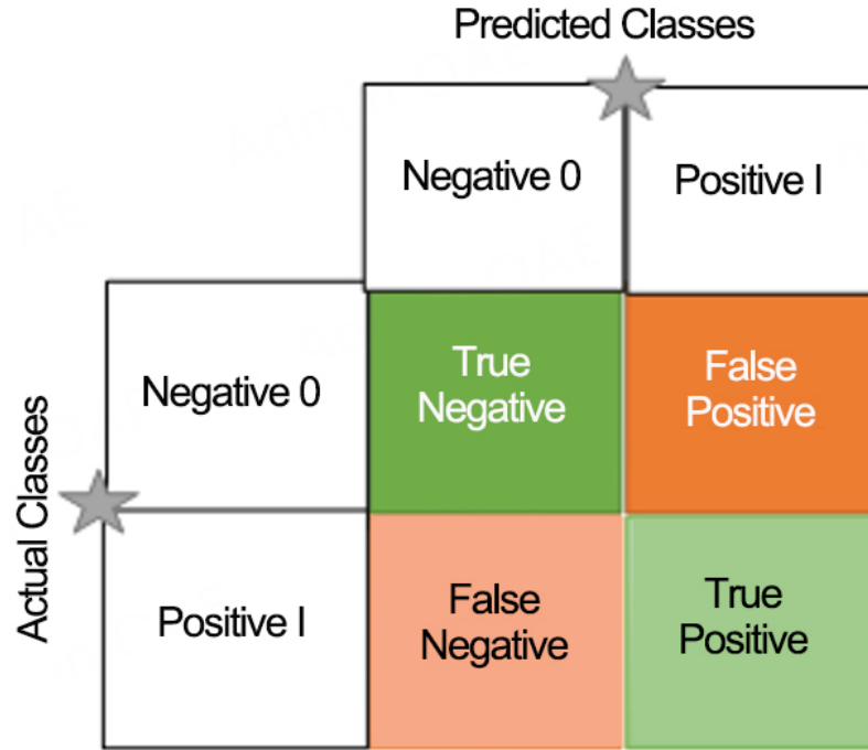
Figure 1. Confusion matrix.
