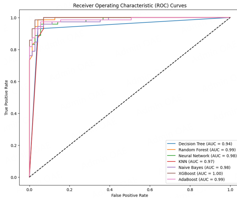
Figure 6. ROC curve.
