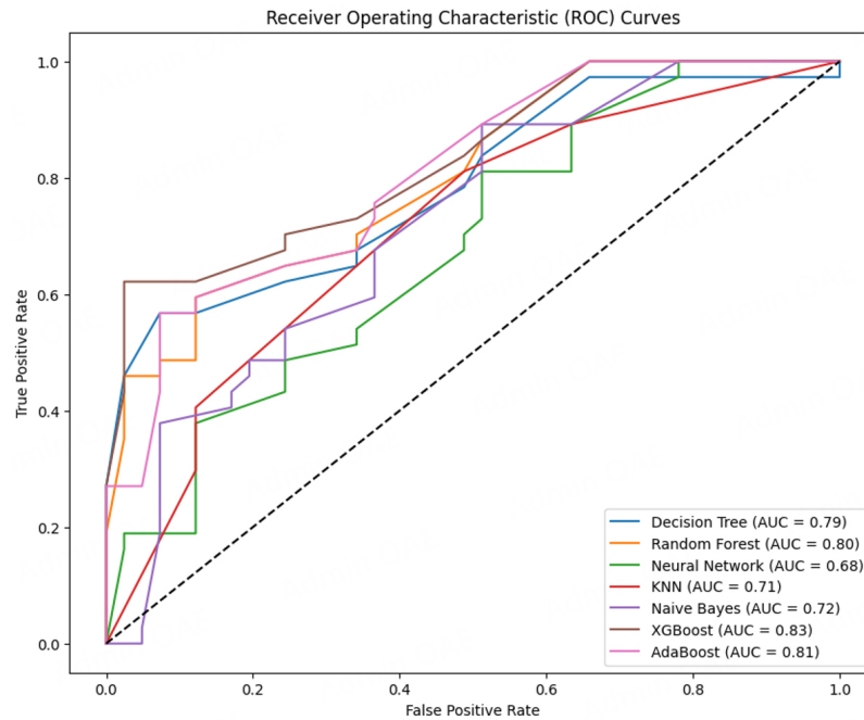
Figure 12. ROC curve.
