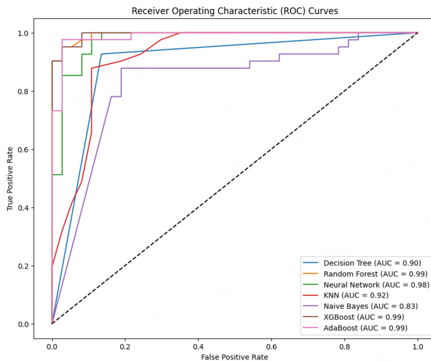
Figure 16. ROC curve.
