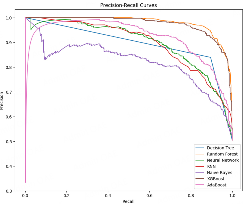
Figure 23. Precision recall curve.
