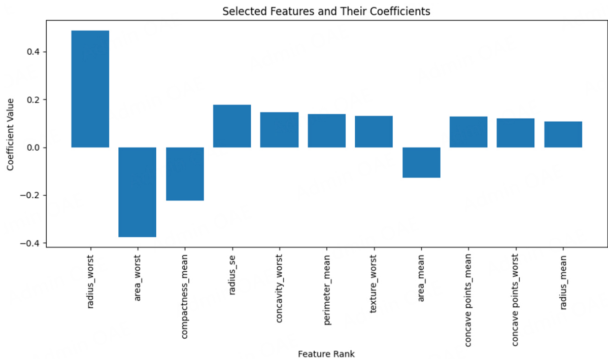
Figure 4. Features selected with their coefficients.
