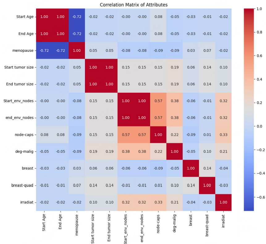
Figure 8. Correlation matrix.
