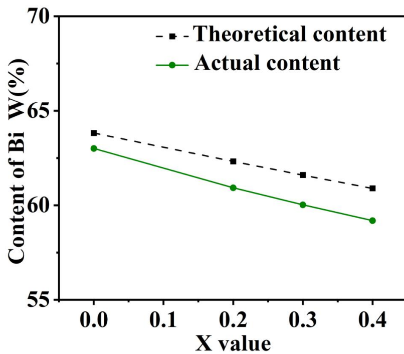
Fig. S2. ICP-MS measurement of Bi content.
