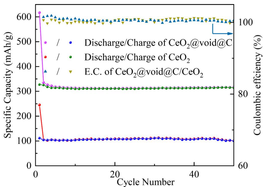
3 Figure S3. Electrochemical cycling performance of the untreated CeO 2 and 4 CeO 2 @void@C anodes for the initial 50 cycles under a current density of 100 mA·g -1 .
