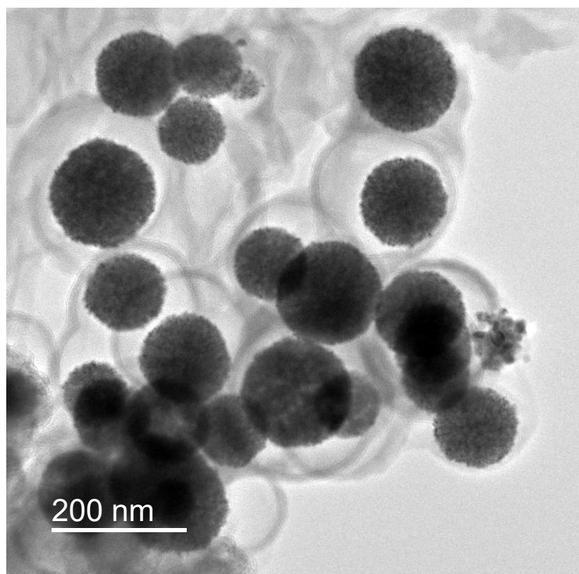
Figure S1. TEM image of the as-prepared CeO 2 @void@C mesoporous microspheres after electrochemical cycling.
