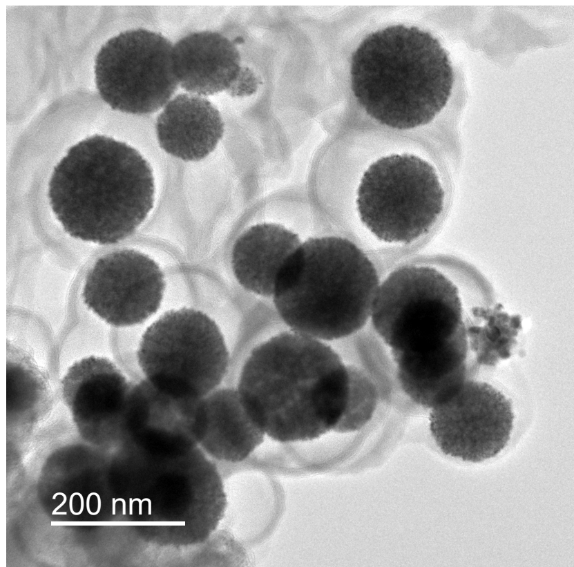
1 2 Figure S1. TEM image of the as-prepared CeO 2 @void@C mesoporous microspheres 3 after electrochemical cycling.
