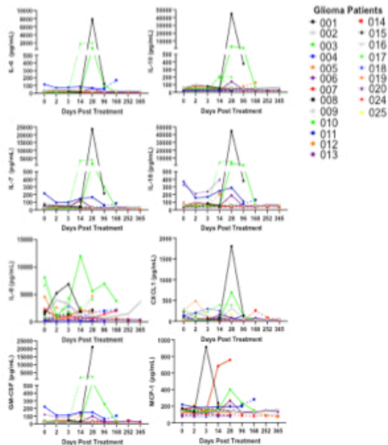
Supplemental Figure 6. Analysis of peripheral blood for correlates of tumor immune responses. Immune function was characterized using multianalyte ELISA to determine cytokine and chemokine expression in peripheral blood and plasma obtained at specific time points after M032 treatment.
