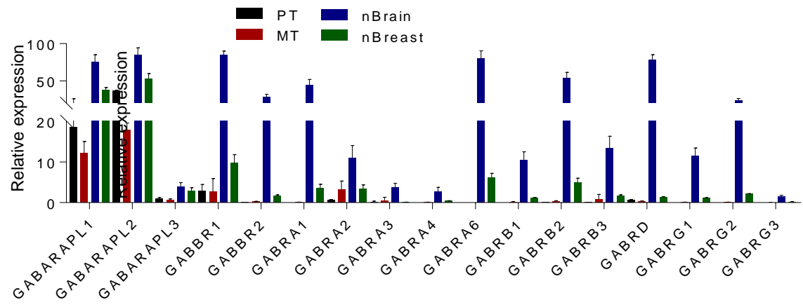
Figure S5: Expression of GABA receptors and subunits in primary breast cancer (PT), Breast to brain metastatic (MT), normal breast (nBreast), and normal brain (nBrain) tissues.
