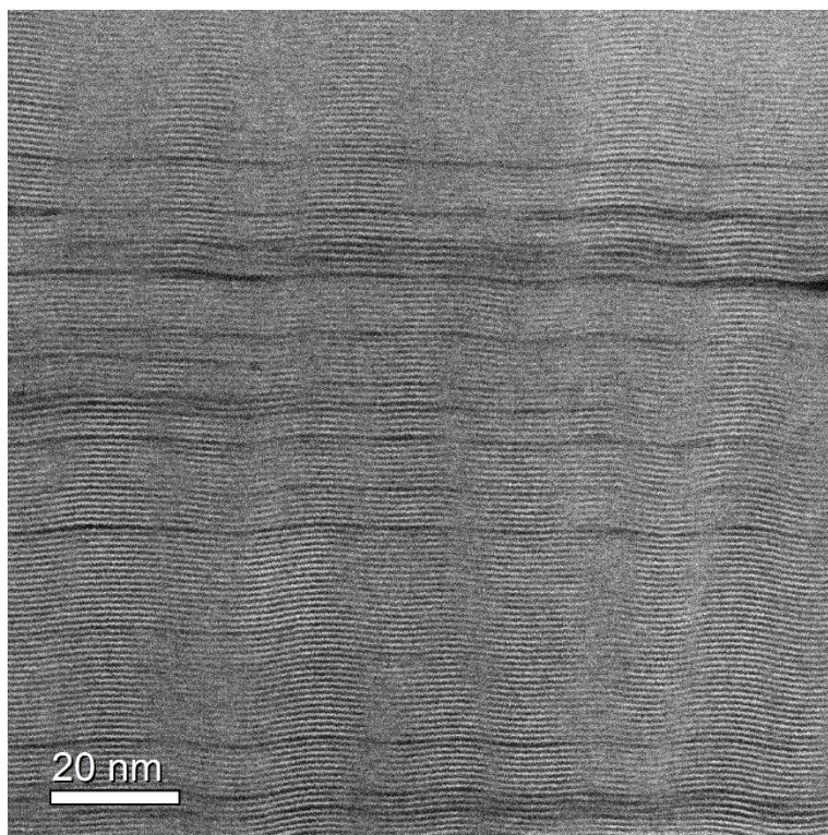
Supplementary Figure 4. HAADF-STEM figure of \text{TiS}_2/\text{HA}/\text{H}_2\text{O} .
